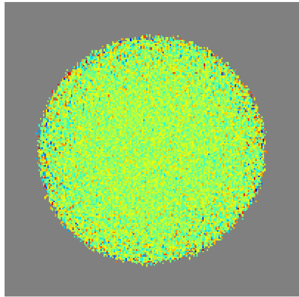
140.0 GHz - U Residual
