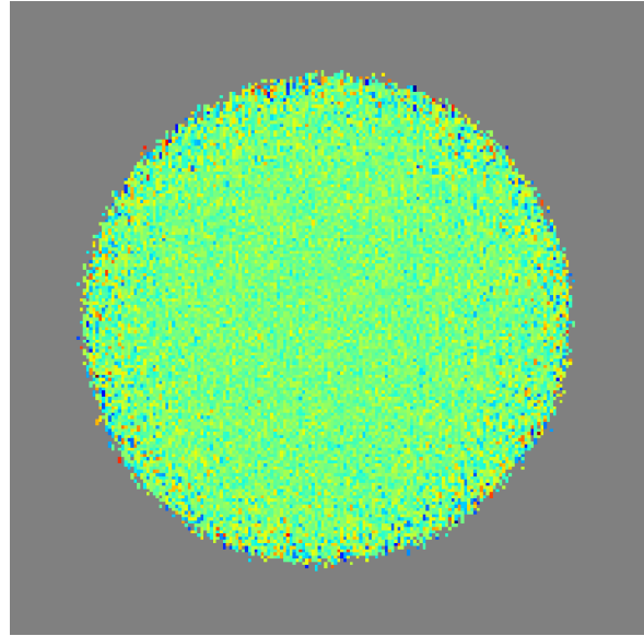
233.0 GHz - U Residual
