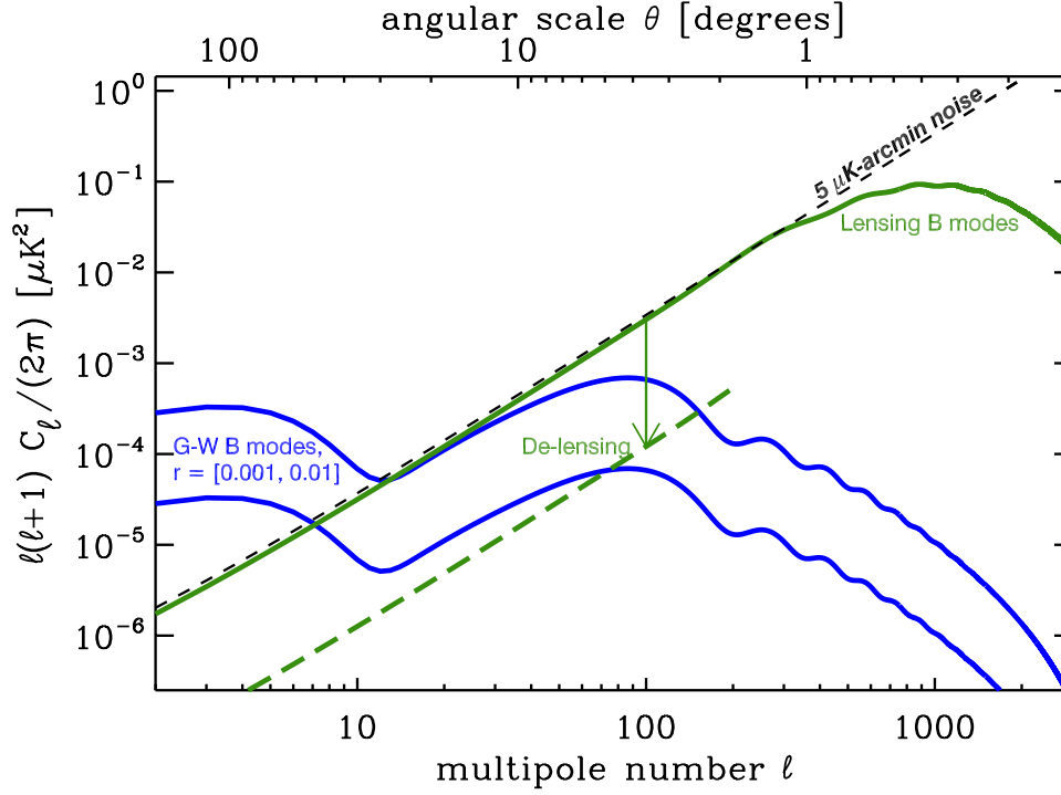
Figure 1.15: Blue curves are the power spectrum of B-modes for different value of the tensor-to-scalar ratio (0.01 and 0.001). The green curve is the power spectrum of lens-induced E-to-B mixing. Delensing can reduce the amplitude of this effect by large factors (green dashed curve) yielding lower effective noise in B-mode maps. Taken from [49].
