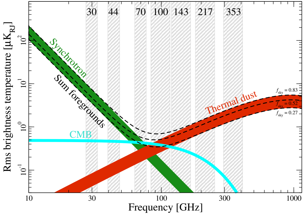
Figure 1.16: Planck’s measurements of polarization amplitude rms as a function of frequency for polarised synchrotron emission (green), polarised thermal dust emission (red) and CMB polarisation (cyan). The dashed black lines indicate the sum of foregrounds evaluated over three different masks with f_{\text{sky}} = 0.83 , 0.52 , and 0.27 . The widths of the synchrotron and thermal dust bands are defined by the largest and smallest sky coverages. Taken from [51].
