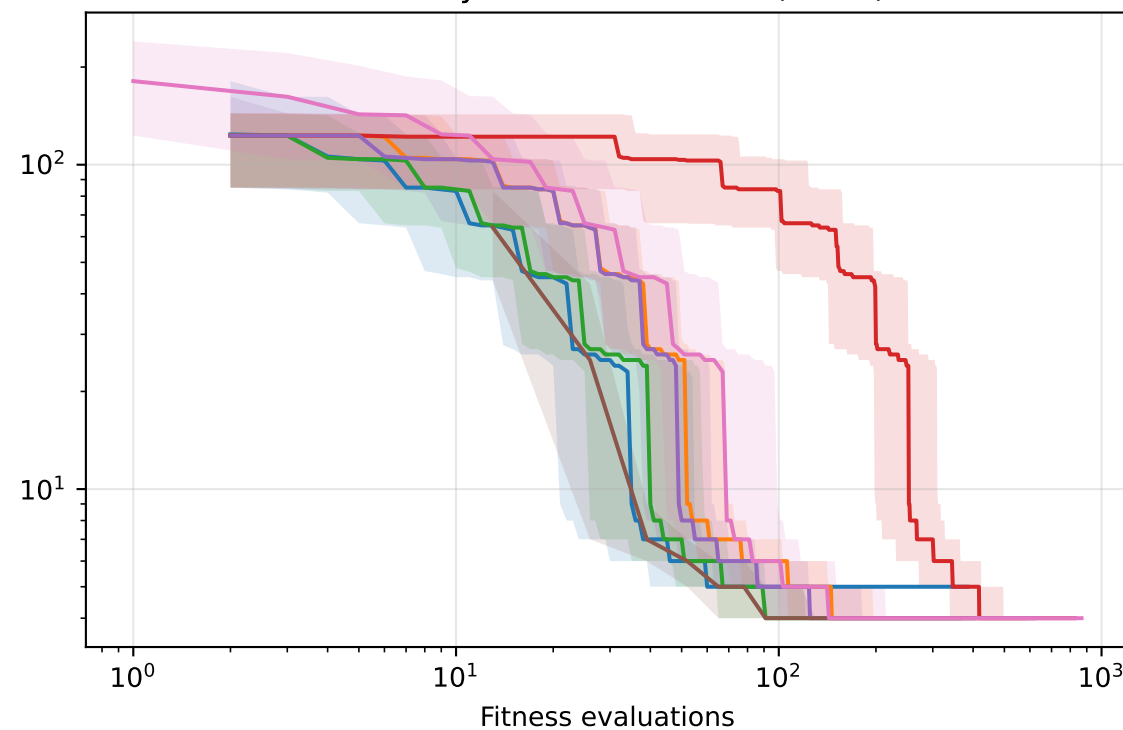
MIVS Anytime Performance (n=72)
