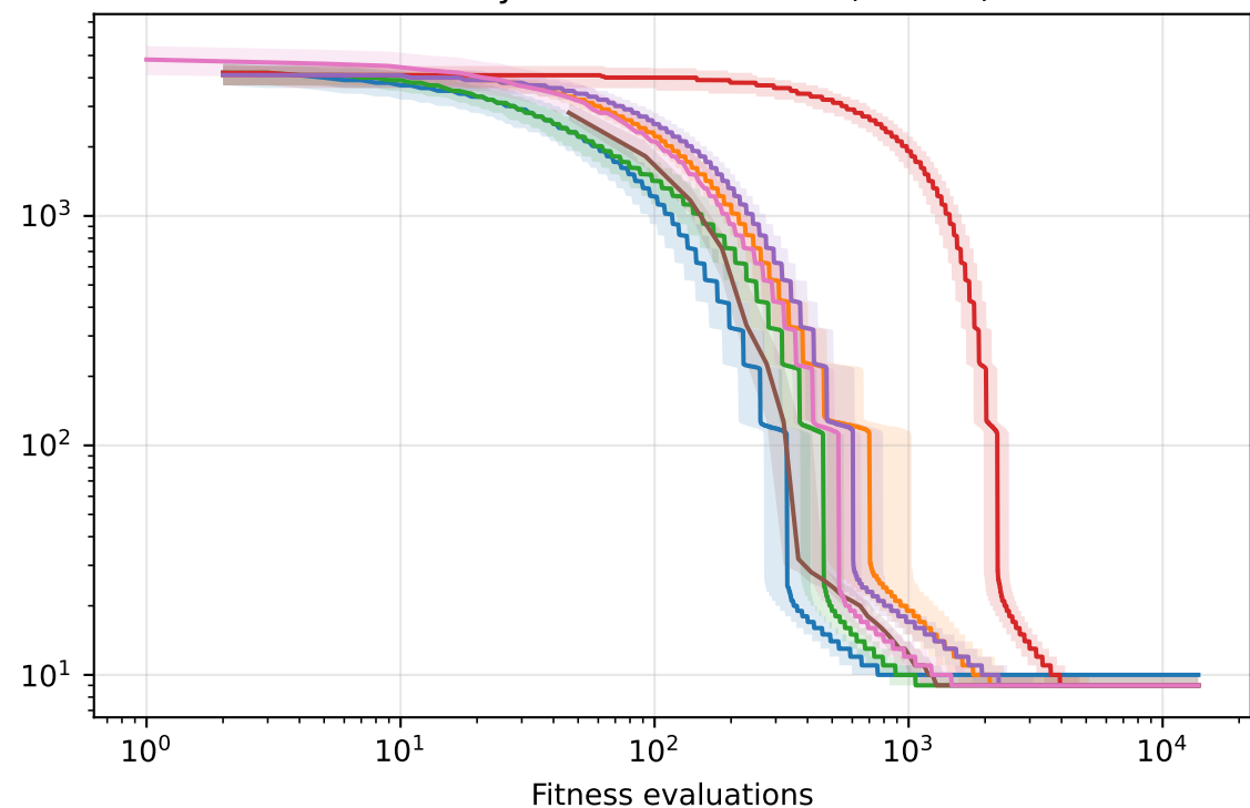
MIVS Anytime Performance (n=100)
