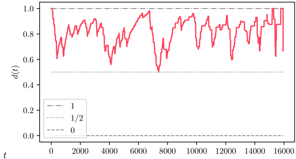
(2+1) -DEGA( n = 200, \lambda = n^{2/3} )
