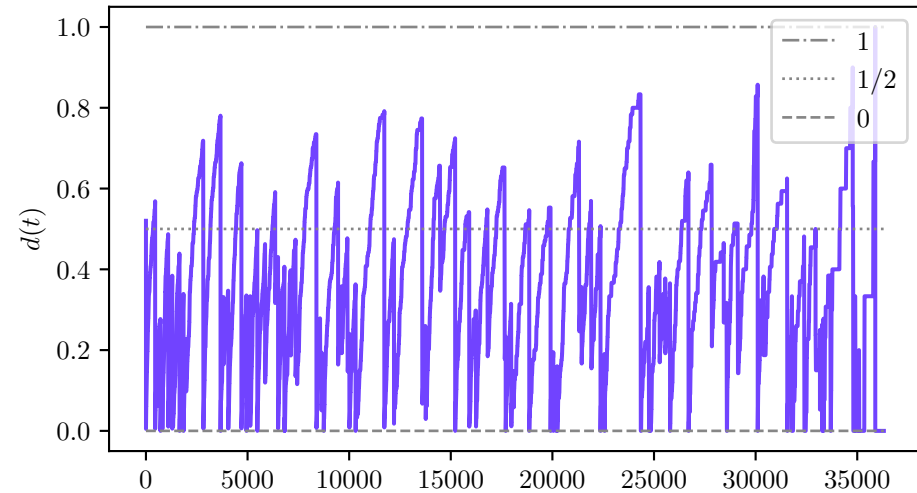
(2+1) -GA( n = 200 )
