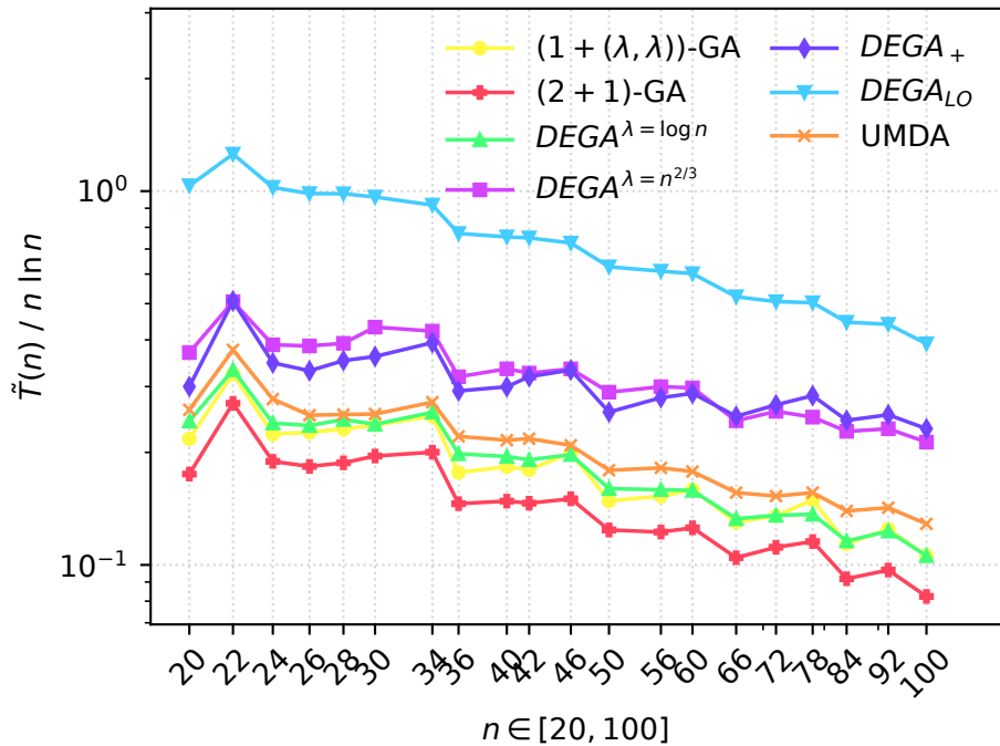
Median
