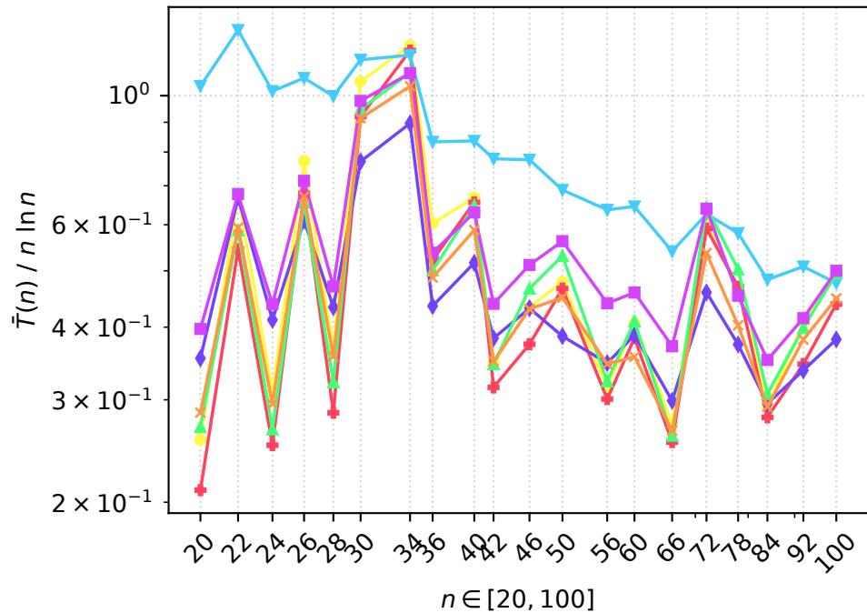
Mean
