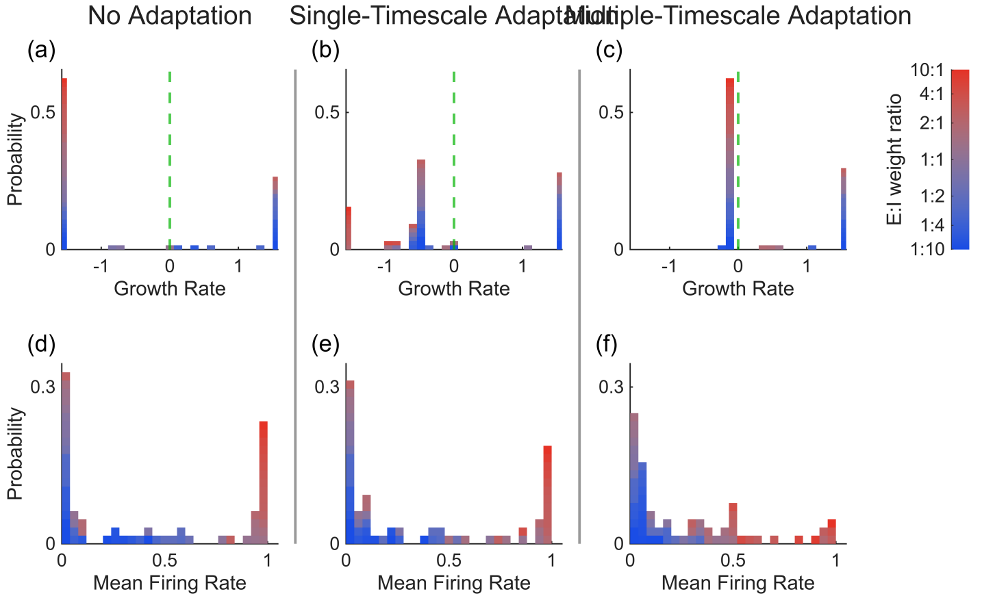
Figure 5: fig_EI_weights_param_space/Fig_EI_Weights_ParamSpace.png
