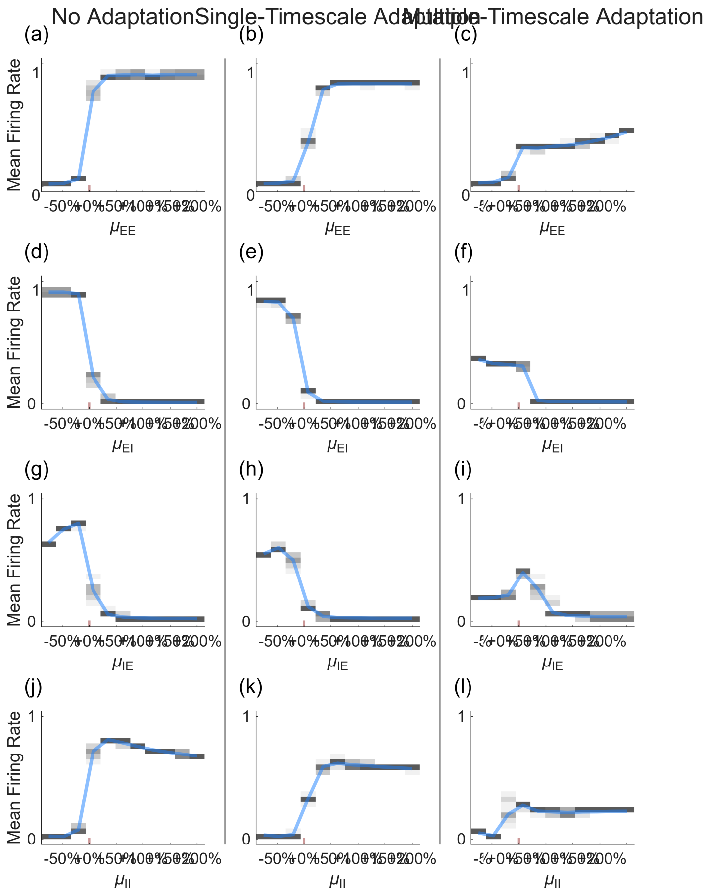
Figure 18: fig_sensitivity_analysis_allStd/fig_sensitivity_mean_rate_mu.png
