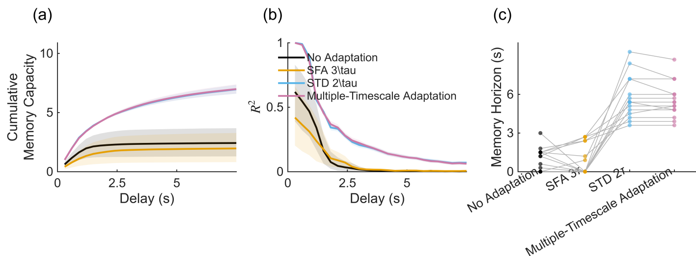
Figure 12: fig_memory_capacity/Fig_Memory_Capacity.png
