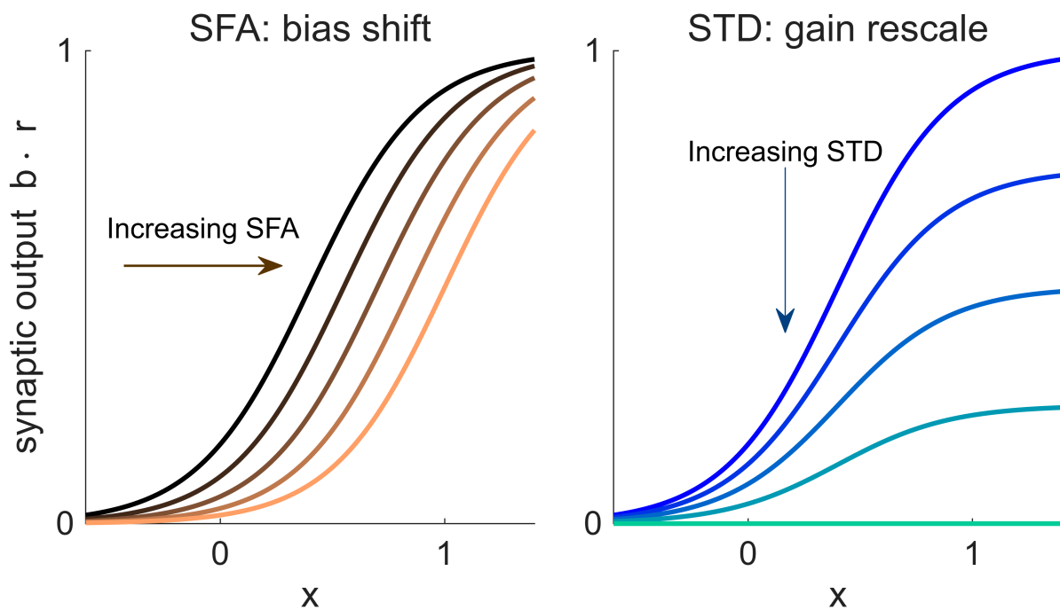
Figure 9: fig_FI_curve/Fig_FI_curve.png
