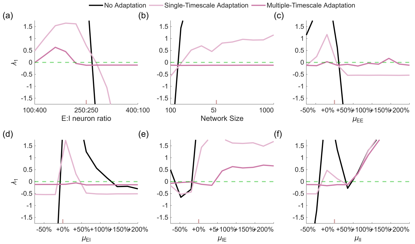
Figure 19: fig_sensitivity_medians/Fig_Sensitivity_LLE_medians.png
