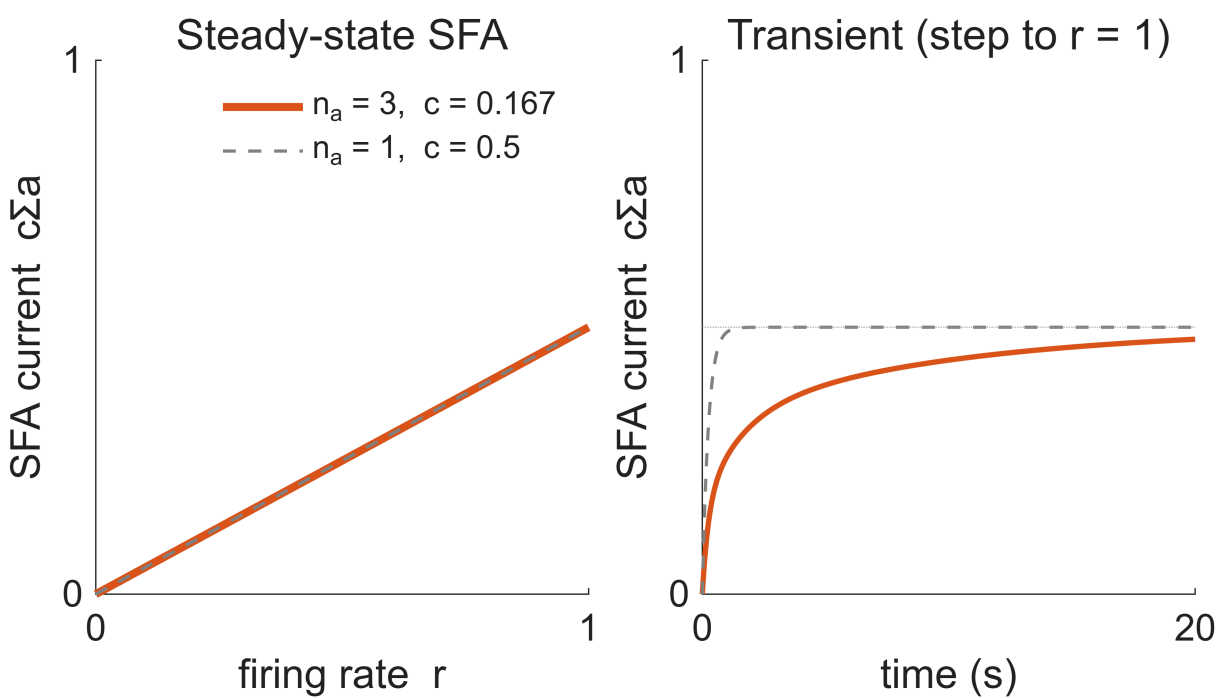
Figure 22: fig_SFA_steady_state/Fig_SFA_steady_state.png
