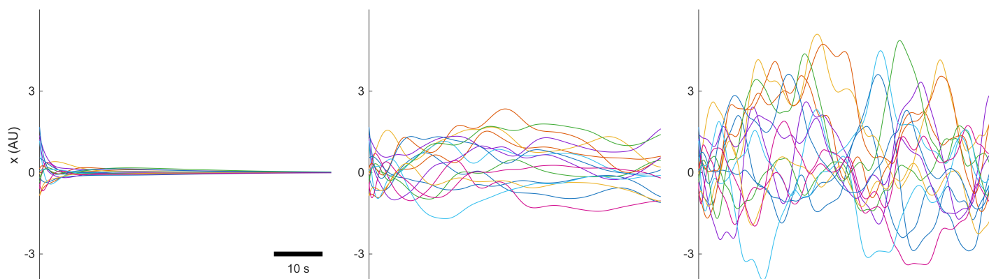
Figure 11: fig_introduutory_concepts/statetraces/panelA_bottom_traces.png
