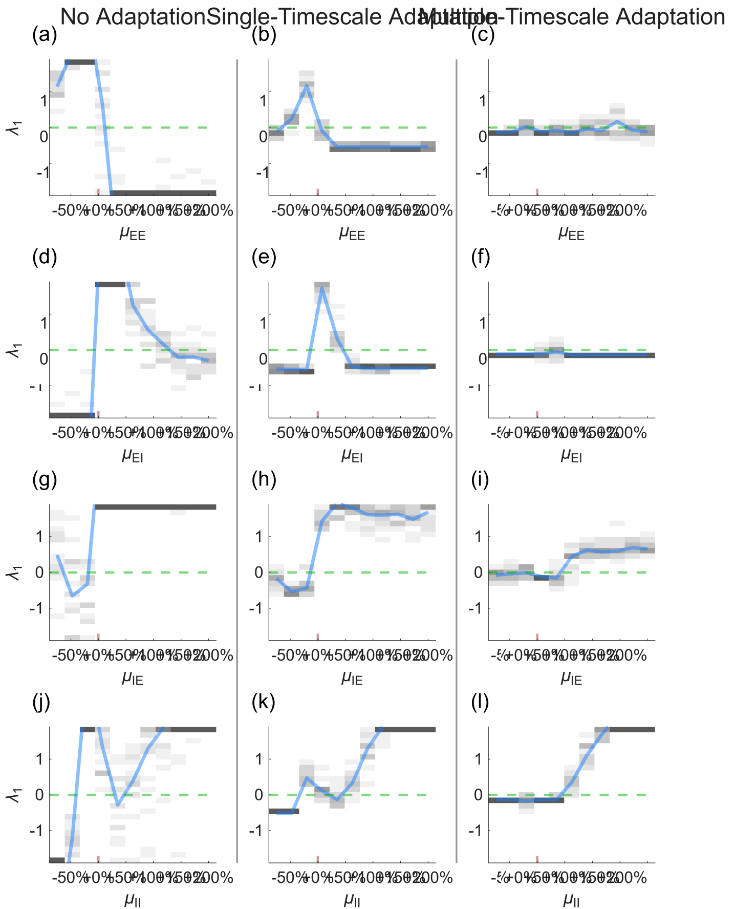
Figure 16: fig_sensitivity_analysis_allStd/Fig_Sensitivity_LLE_mu.png
