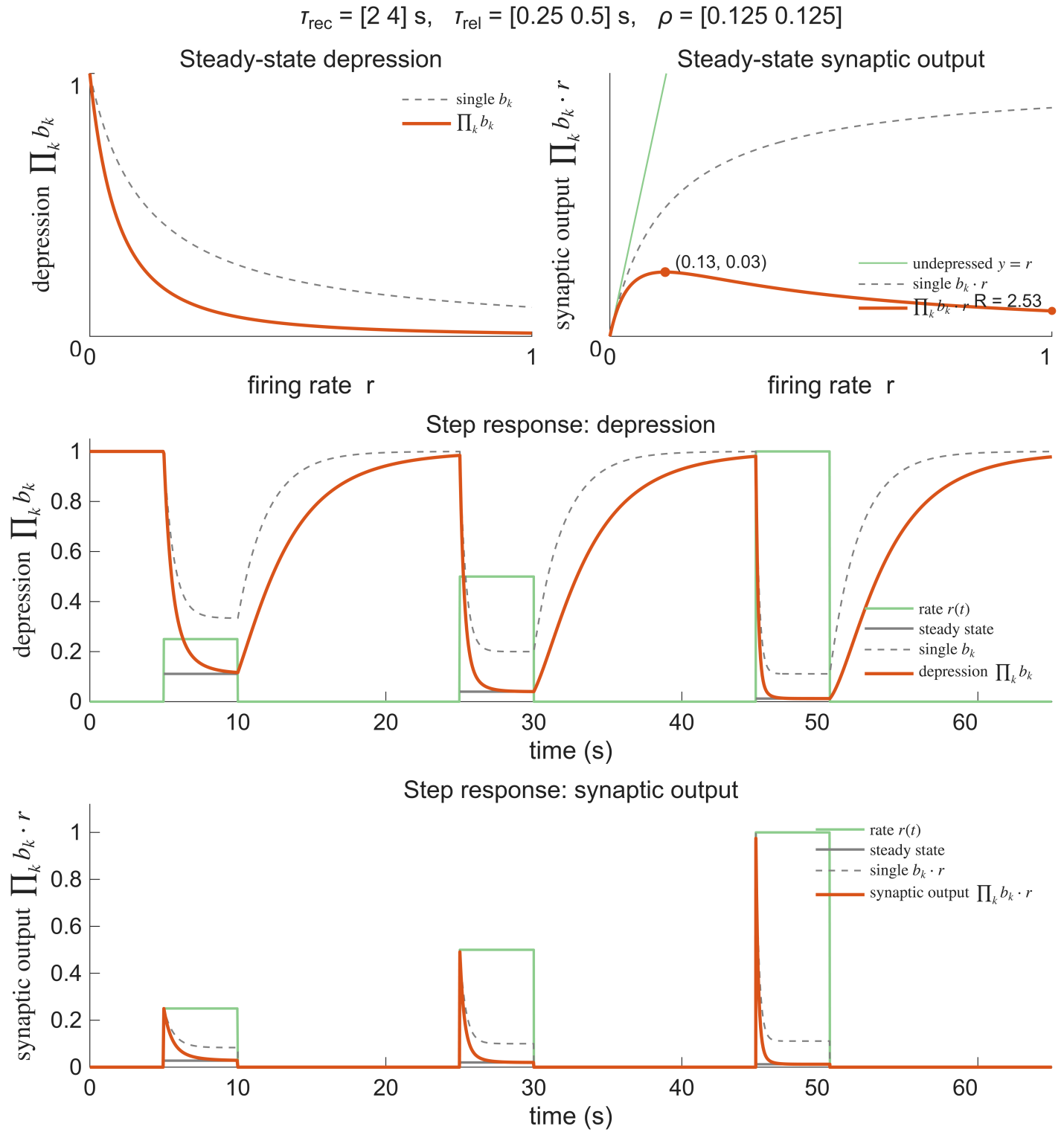
Figure 23: fig_STD_steady_state/Fig_STD_steady_state.png
