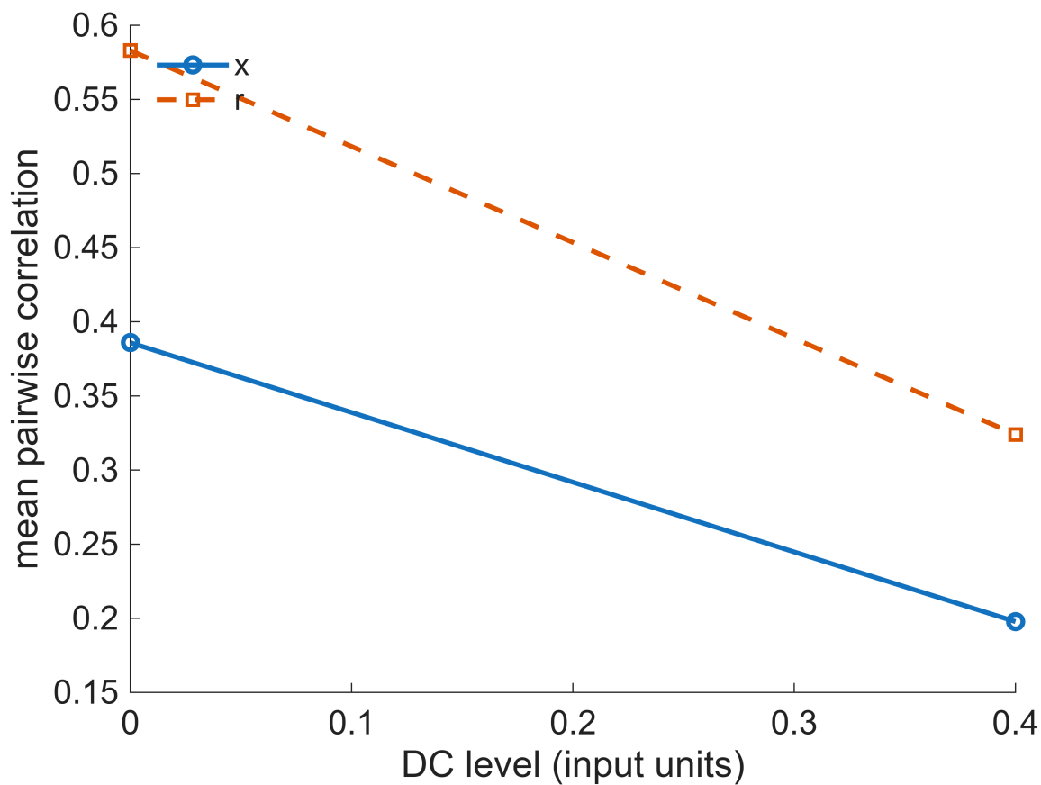
Figure 25: fig_stim_engages_adaptation/bursting_synchrony.png
