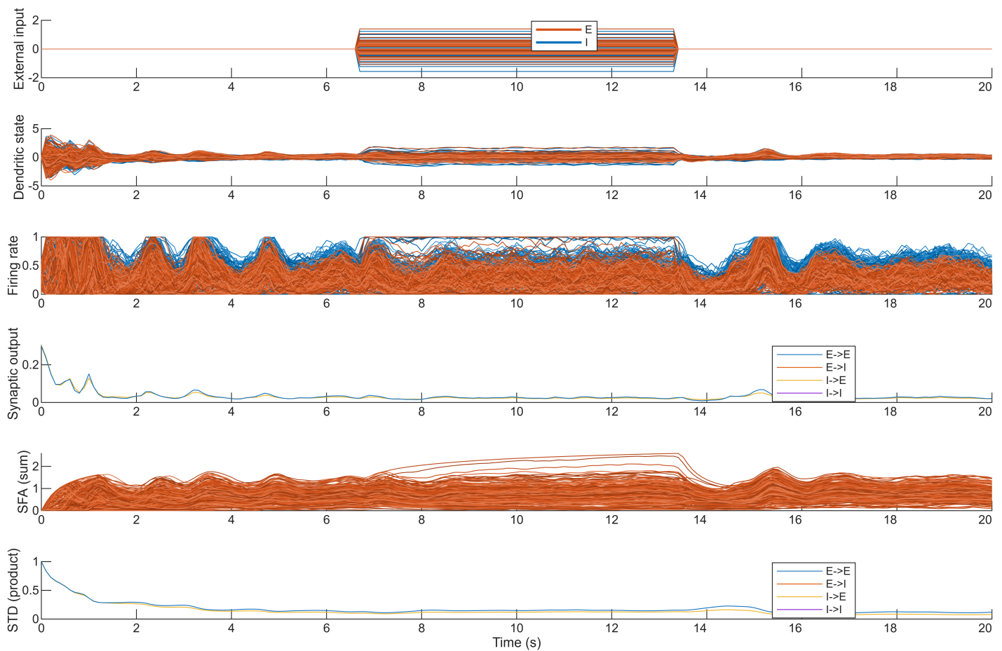
Figure 8: fig_example_timeseries/fig_example_timeseries.png
