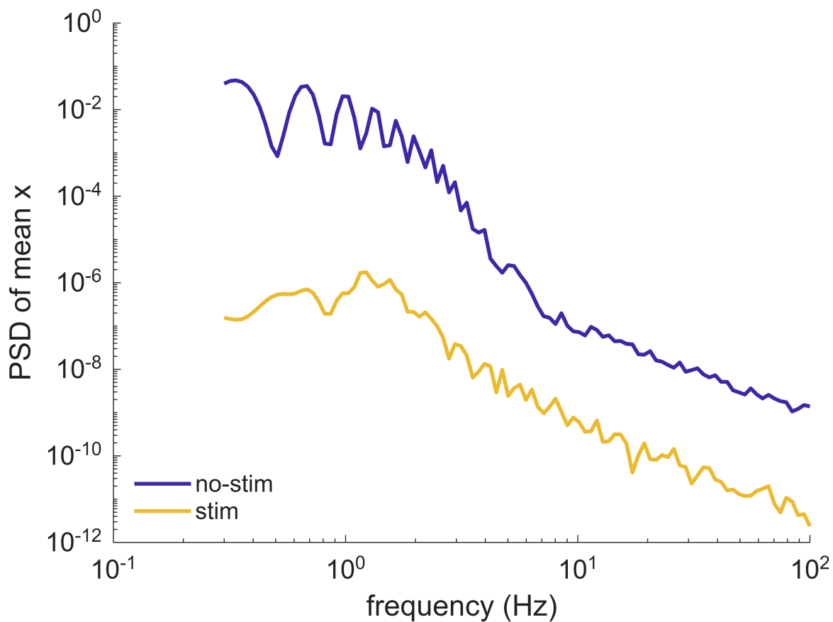
Figure 24: fig_stim_engages_adaptation/bursting_psd.png
