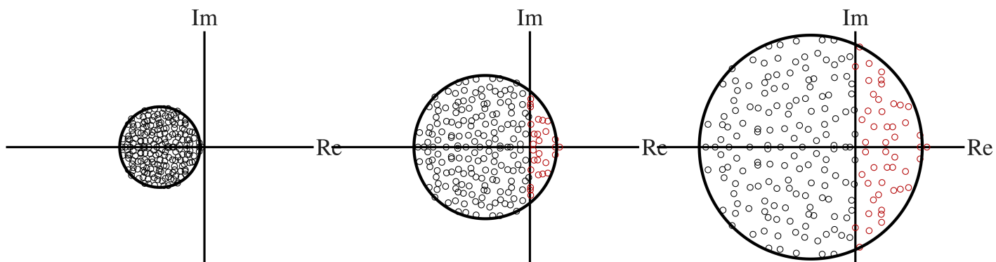
Figure 10: fig_introduutory_concepts/eigenspectra/panelA_eigenspectrum.png
