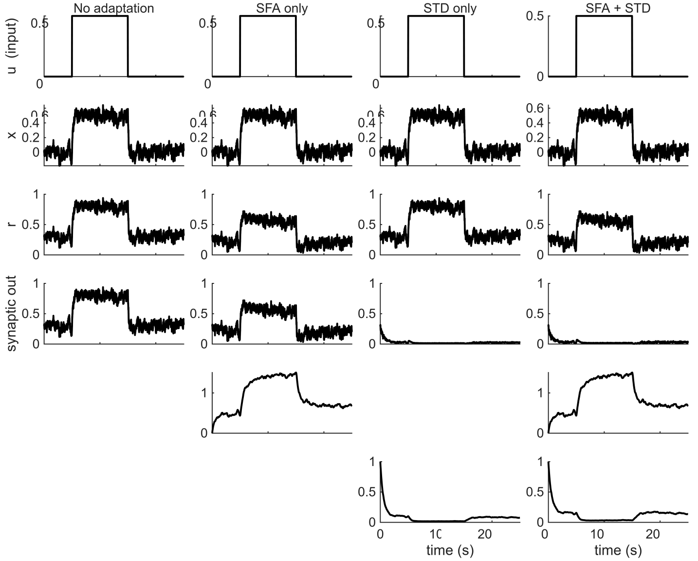
Figure 1: fig_adaptation_methods/Fig_single_neuron_SFA_STD.png
