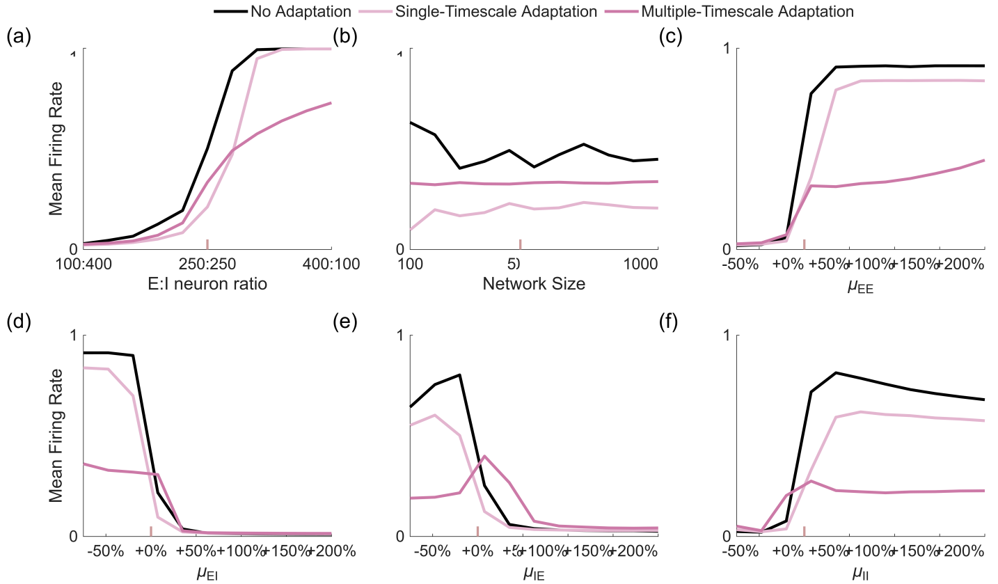
Figure 20: fig_sensitivity_medians/Fig_sensitivity_mean_rate_medians.png
