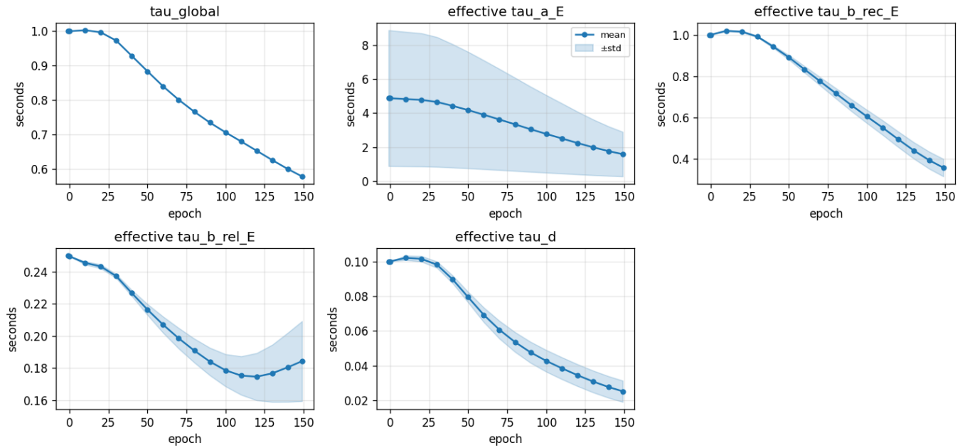
alpha-ramp-150e — effective time constants (srnn-e-only-skip-per-neuron)
