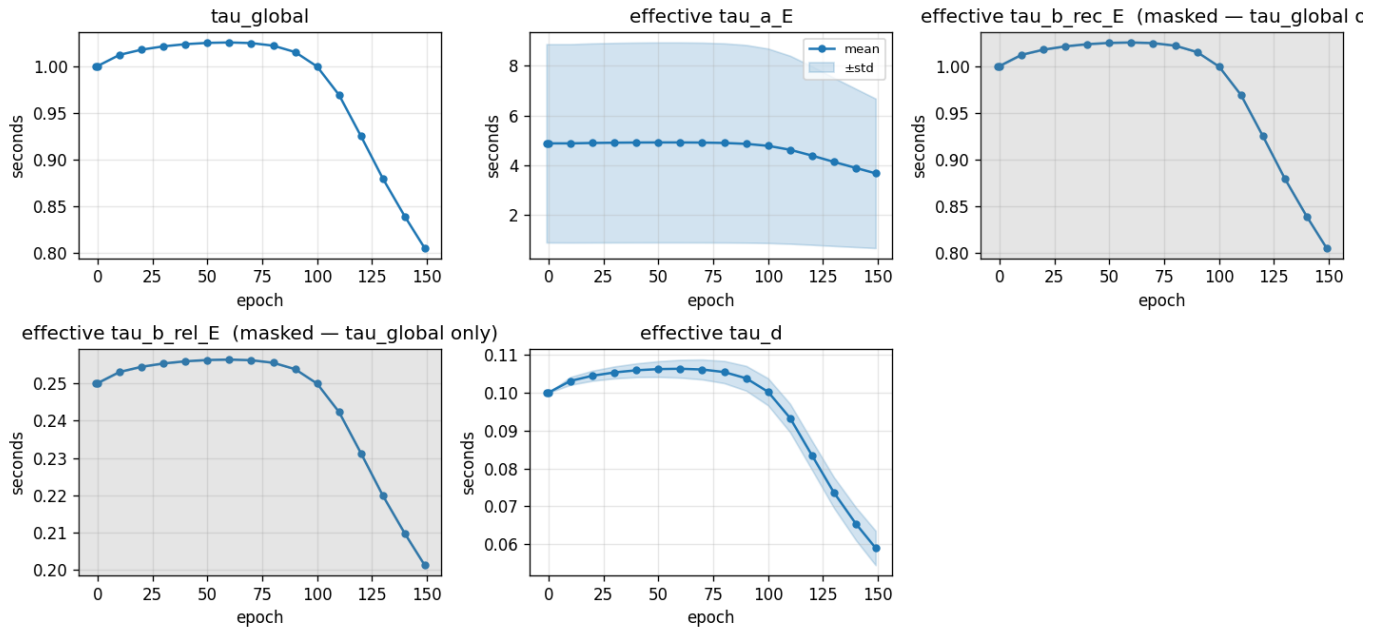
alpha-ramp-150e — effective time constants (srnn-sfa-e-only-skip-per-neuron)
