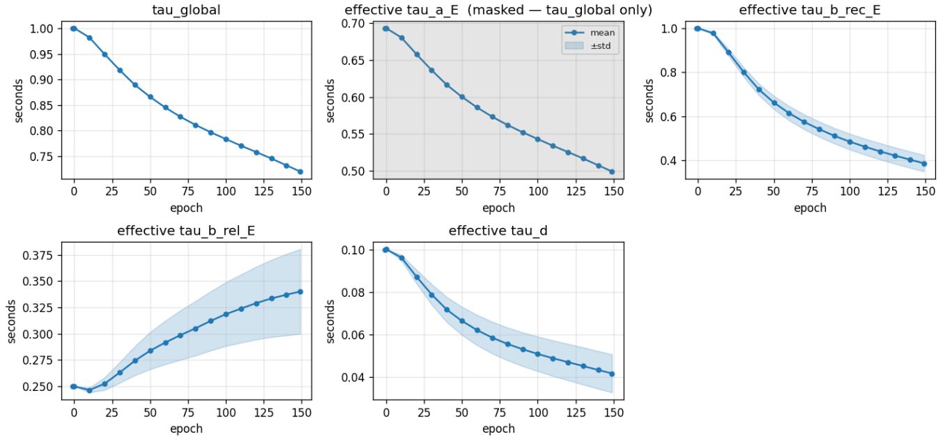
alpha-ramp-150e — effective time constants (srnn-std-e-only-per-neuron)
