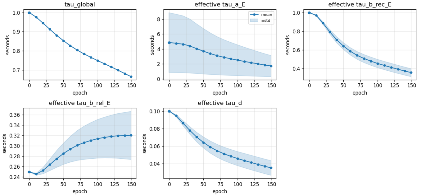
alpha-ramp-150e — effective time constants (srnn-e-only-per-neuron)
