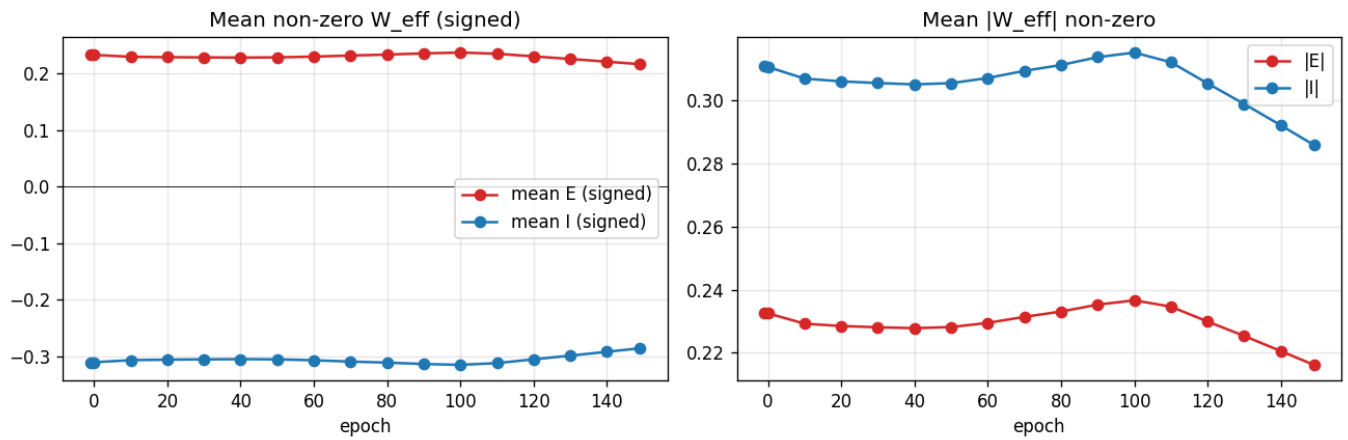
alpha-ramp-150e — recurrent E vs I weights (srnn-std-e-only-skip-per-neuron)
