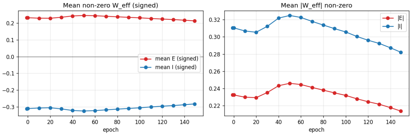
alpha-ramp-150e — recurrent E vs I weights (srnn-e-only-per-neuron)
