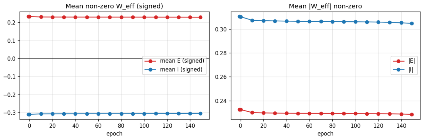
alpha-ramp-150e — recurrent E vs I weights (srnn-sfa-e-only-skip-per-neuron)
