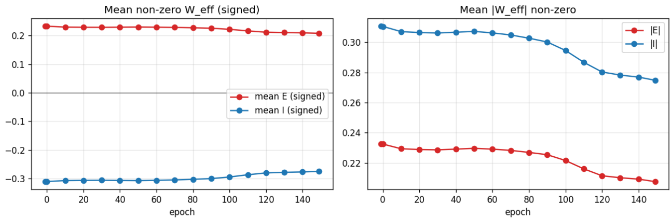
alpha-ramp-150e — recurrent E vs I weights (srnn-e-only-skip-per-neuron)
