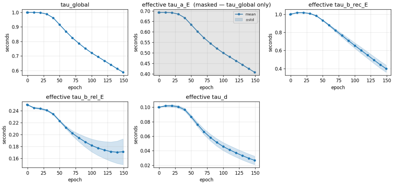
alpha-ramp-150e — effective time constants (srnn-std-e-only-skip-per-neuron)
