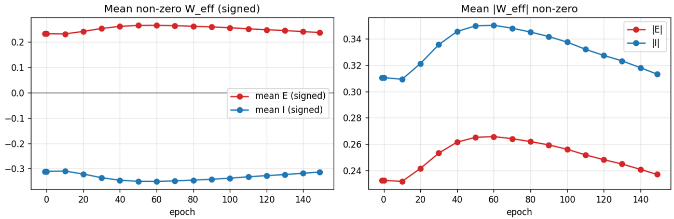
alpha-ramp-150e — recurrent E vs I weights (srnn-std-e-only-per-neuron)
