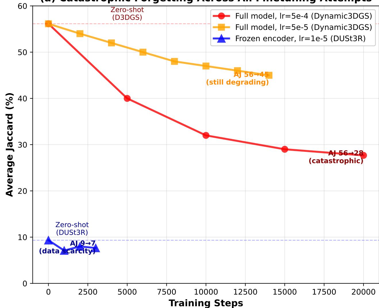
(a) Catastrophic Forgetting Across All Finetuning Attempts
