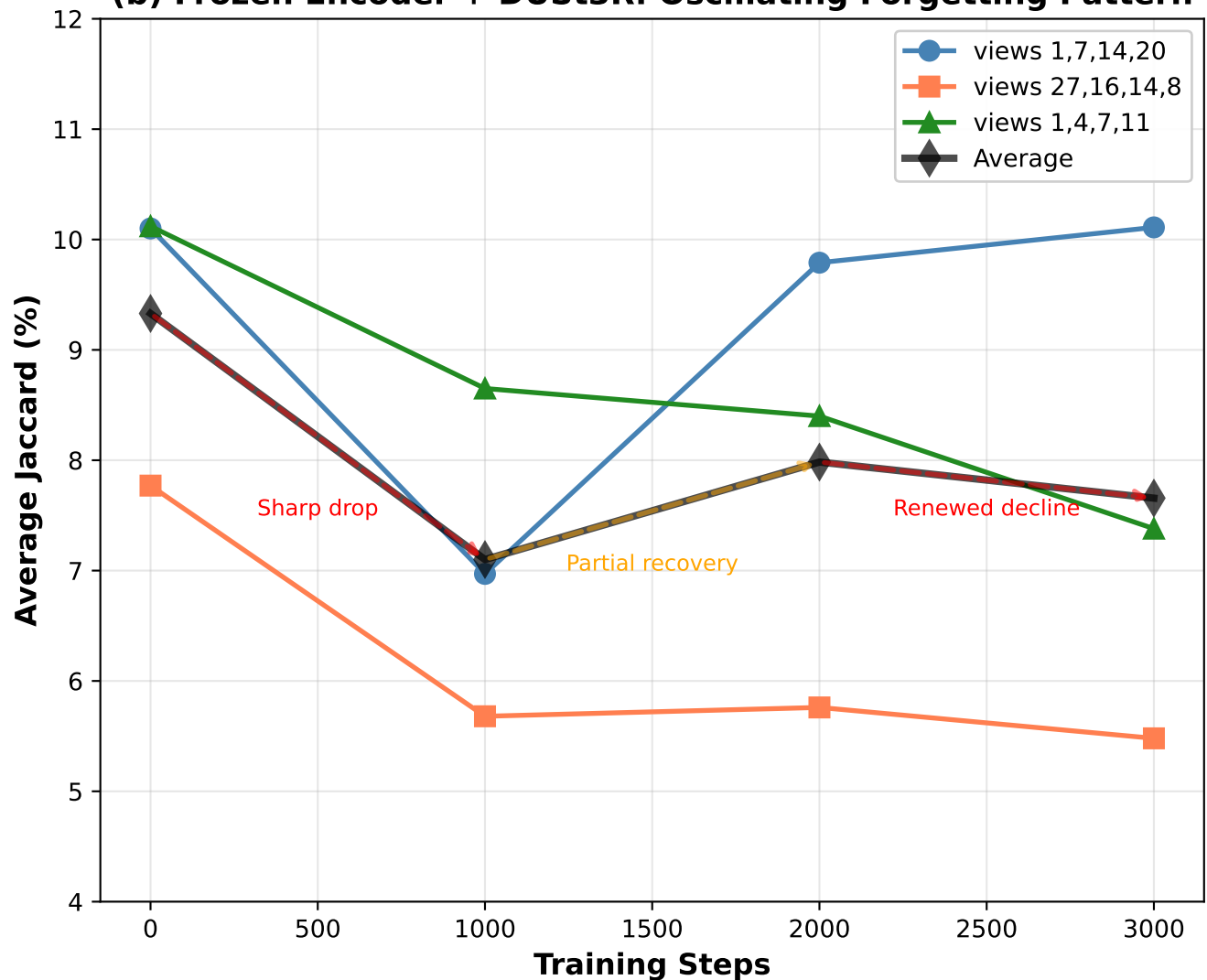
(b) Frozen Encoder + DUST3R: Oscillating Forgetting Pattern
