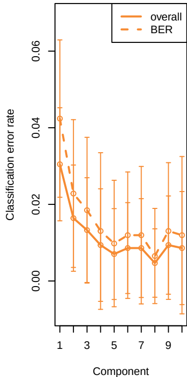
centroids.dist
