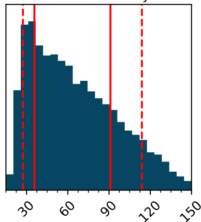
d_{\text{travel}} [pc] Distance traveled by DR1
