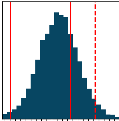
t_{\text{obs}} [Myr] Age at observation
