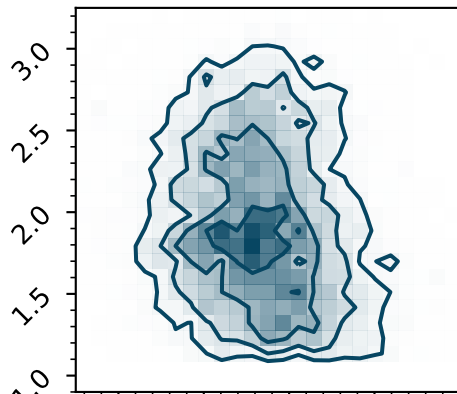
t_{\text{runaway}} [Myr]
