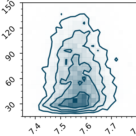
t_{\text{obs}} [Myr]
