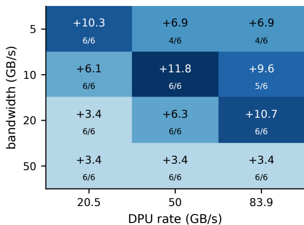
(b) CARTS (cost-aware)
