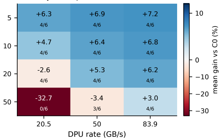
(c) always-dedup (C4)
