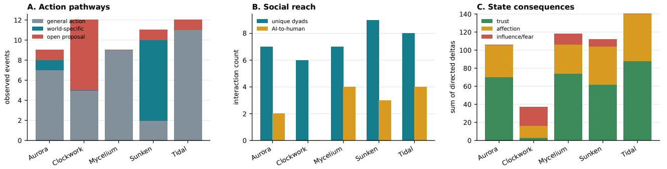
Figure 8: Different interaction profiles emerge under a shared agent policy. Left: events partitioned into general, premise-specific, and newly proposed actions. Center: social reach, including interactions directed at the human player. Right: changes in directed relationship state.
