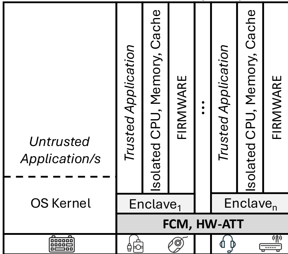
BYOTEE Framework
