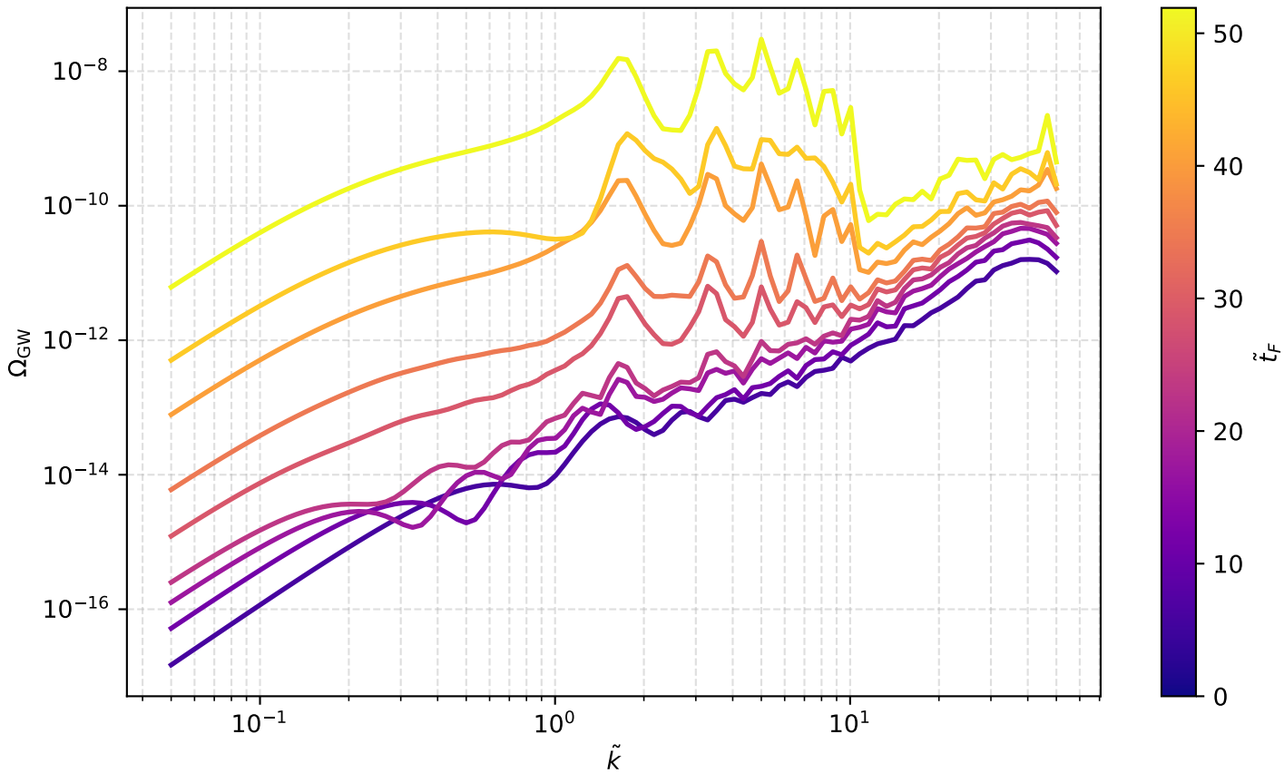
GW spectrum from preheating, q = 5050 , T_{fin} = 7 T_{osc}
