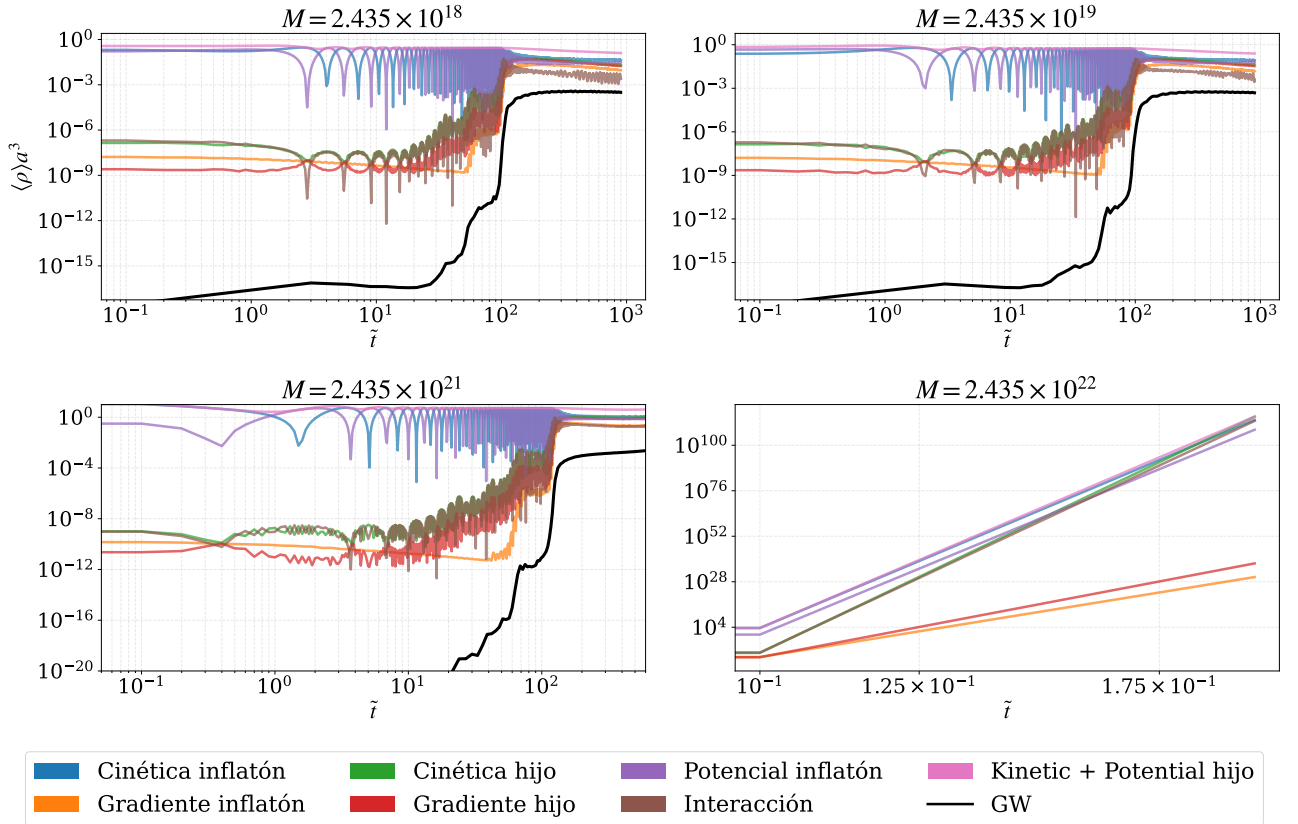
(b) Starobinsky
