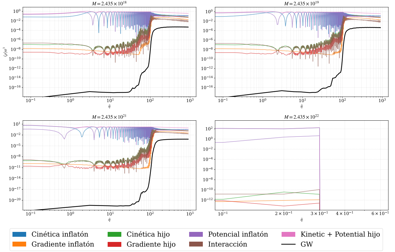
(a) \tanh^2
