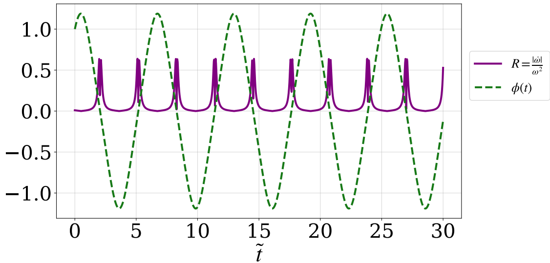
(b) \lambda\phi^4
