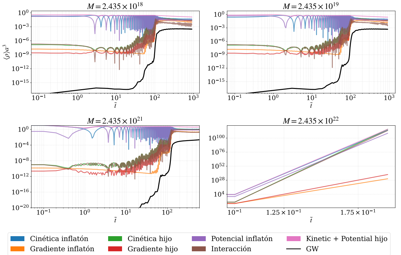
(b) Starobinsky
