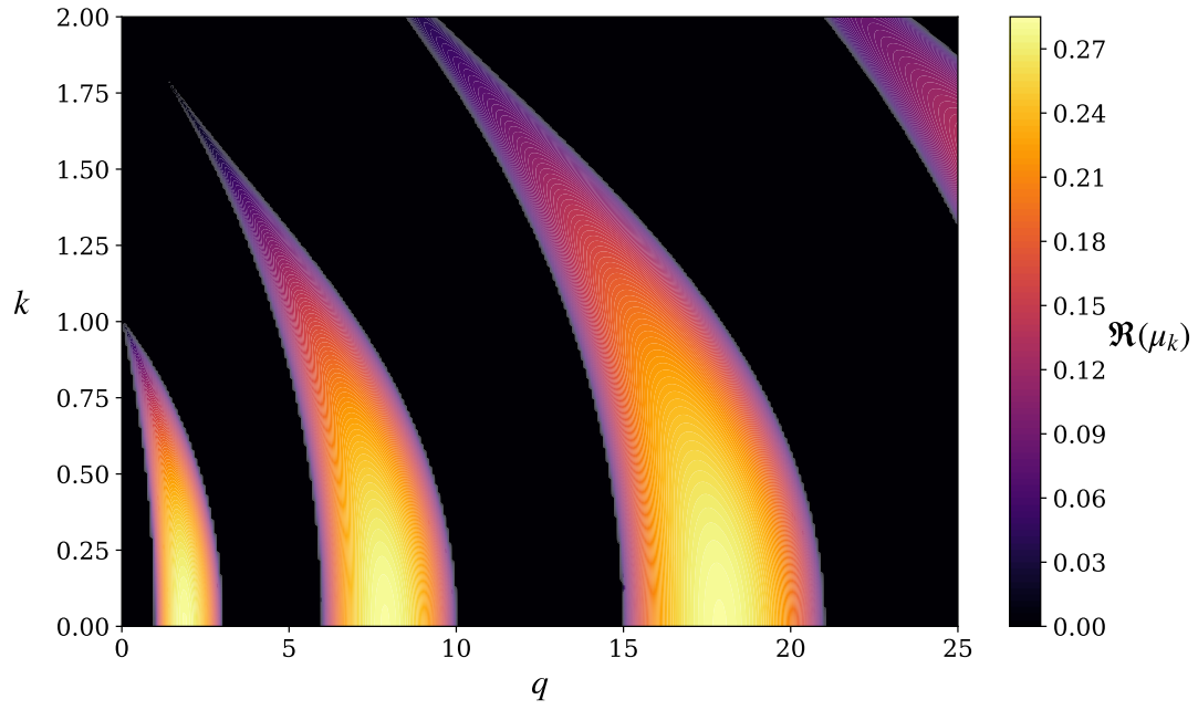
(b) \lambda\phi^4
