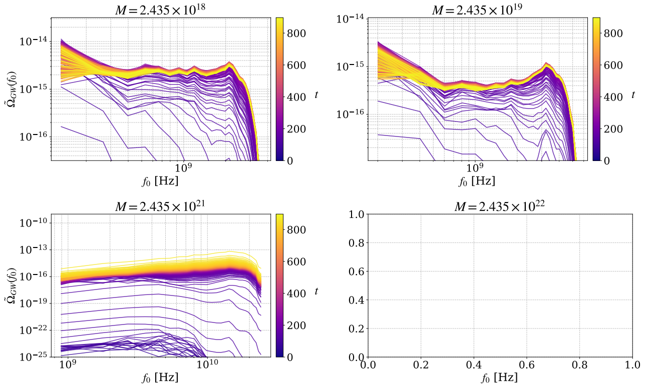
(b) Starobinsky
