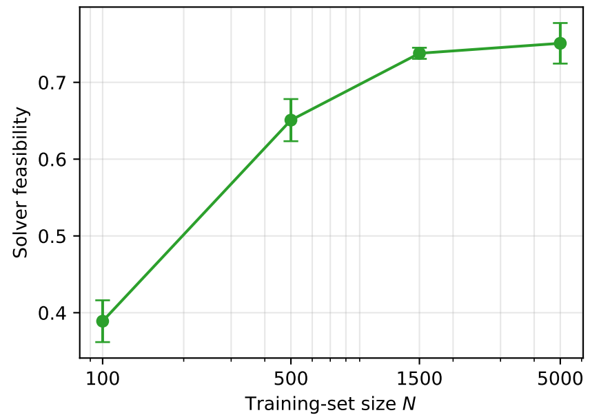
Solver feasibility vs N
