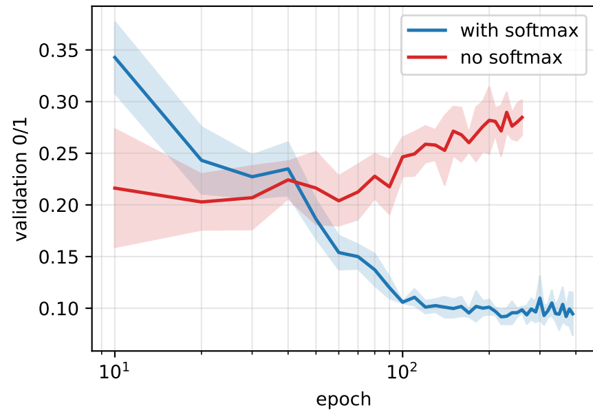
Validation 0/1 vs epoch
