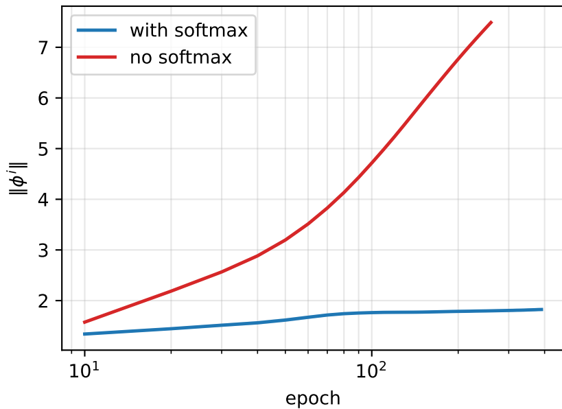
\phi -norm vs epoch
