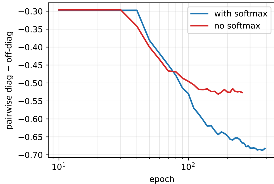
All-different shape (more negative = stronger)
