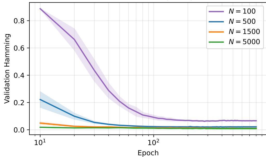
Validation Hamming vs epoch
