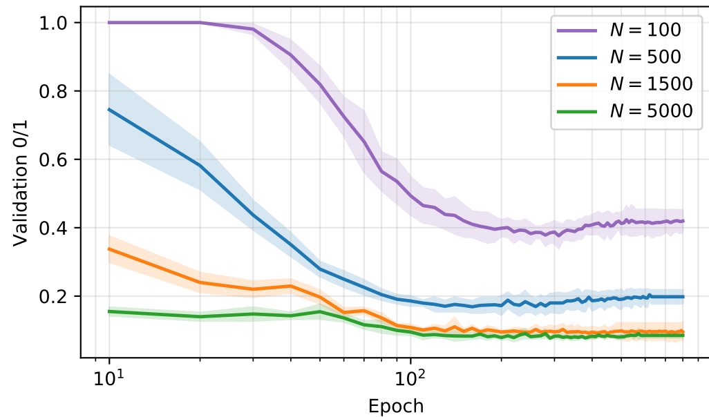
Validation 0/1 vs epoch
