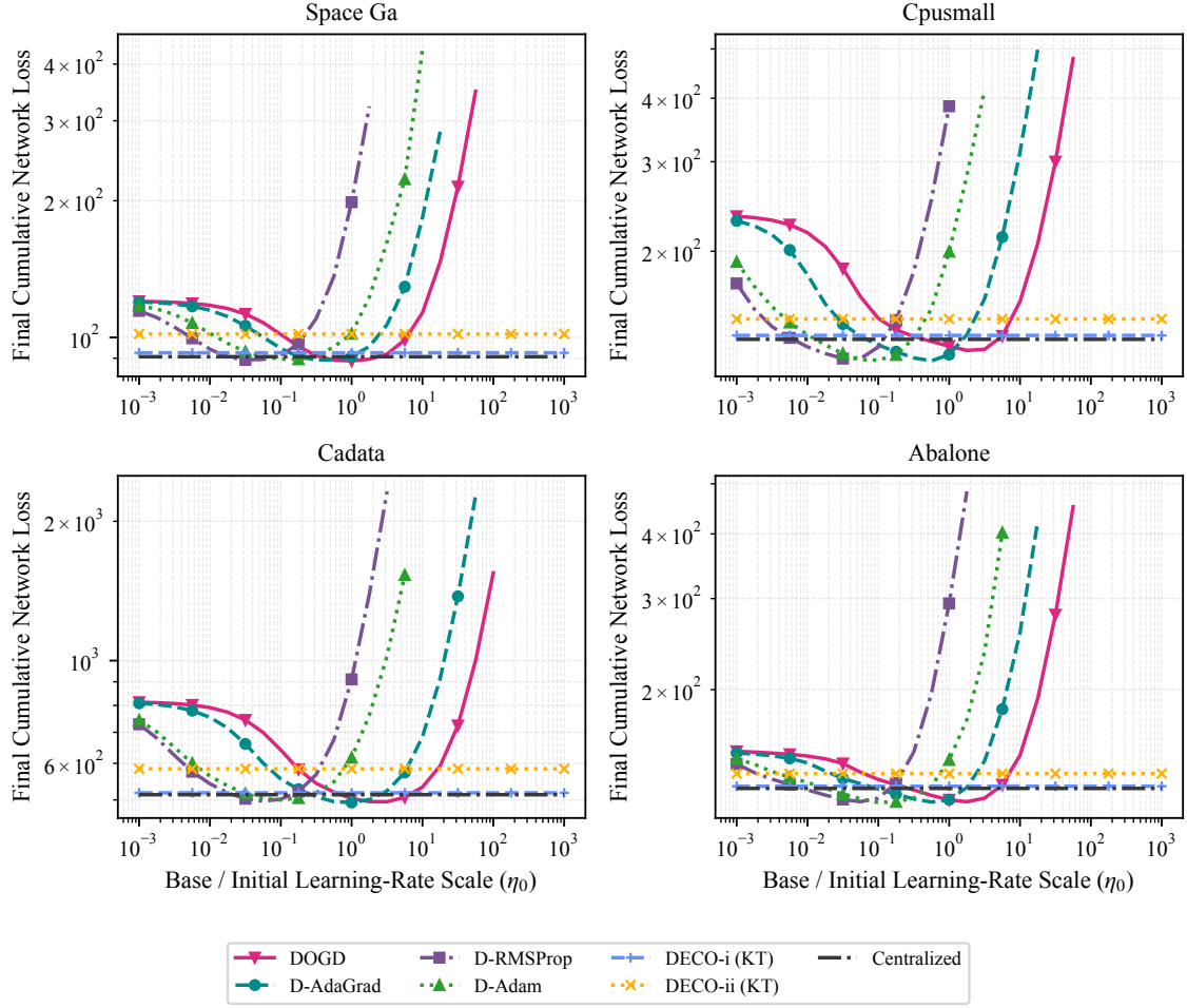
Revised manuscript Fig. 6. Final cumulative network loss on four online LIBSVM streams. Each panel shows the complete 25-value \eta_0 sweep for DOGD, D-AdaGrad, D-RMSProp, and D-Adam on a log-log scale. Horizontal lines show DECO-i/ii (KT) and the centralized reference without learning-rate tuning.
