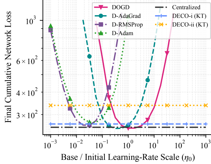
Revised manuscript Fig. 3. Final cumulative network loss on the synthetic online stream across the common base-rate grid \eta_0 \in [10^{-3}, 10^3] . DOGD, D-AdaGrad, D-RMSProp, and D-Adam are swept over all 25 values; the horizontal lines are the untuned DECO-i/ii (KT) and centralized references.
