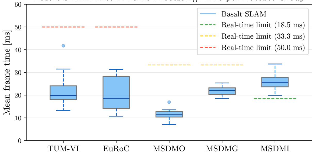
Basalt SLAM: Mean Frame Processing Time per Dataset Group
