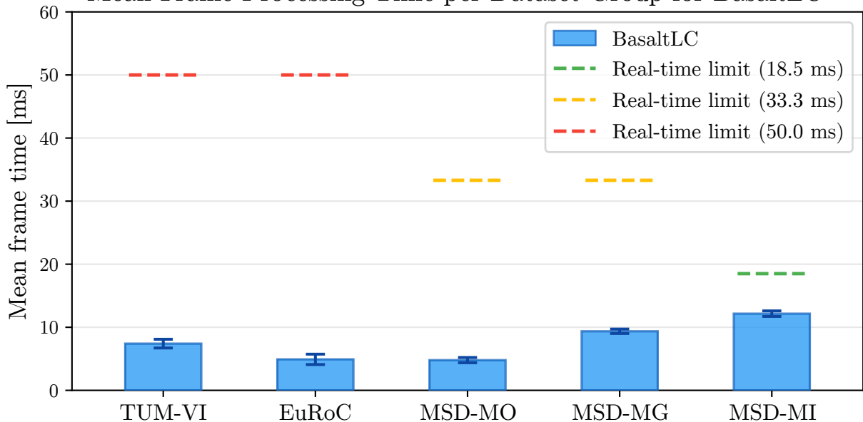
Mean Frame Processing Time per Dataset Group for BasaltLC
