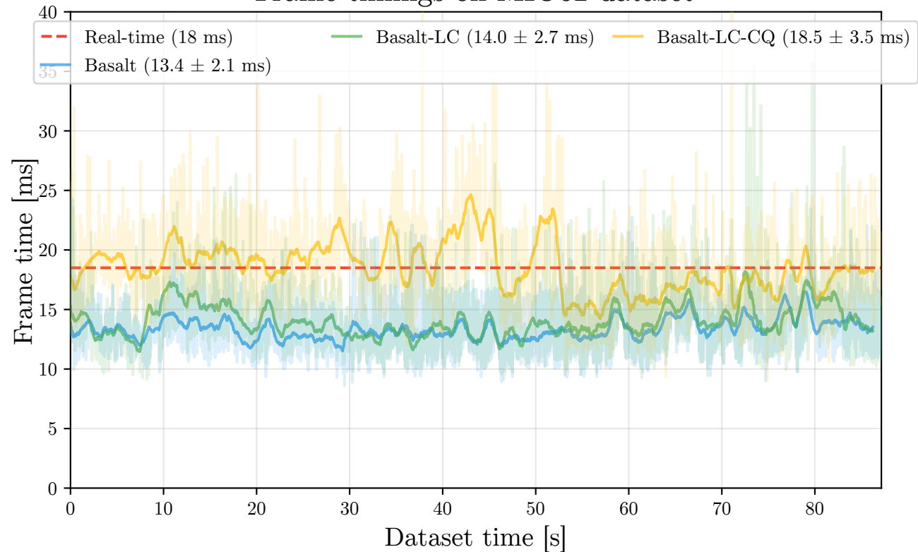
Frame timings on MIO02 dataset
