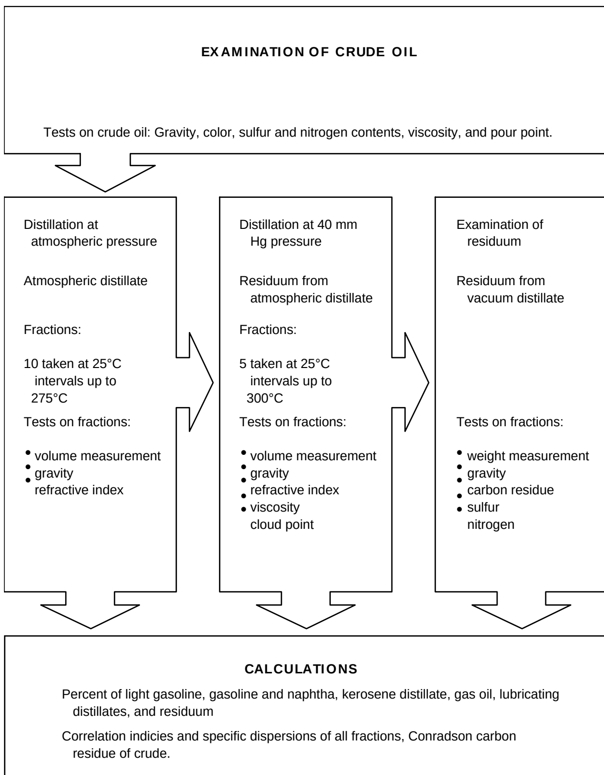
Figure 1-1 Procedure for Crude Oil Analysis
