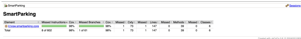
Figura 17: Report JaCoCo – totale (solo package core)
