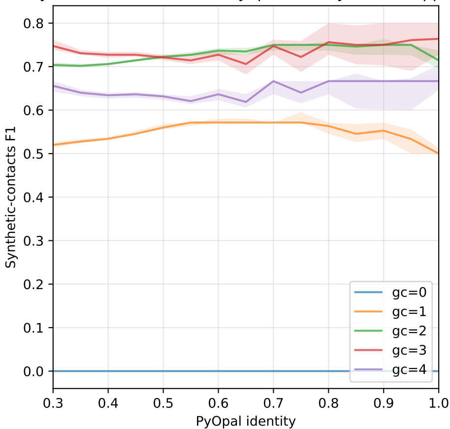
Synthetic-contacts F1 vs PyOpal identity, bootstrapped
