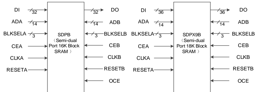
Figure 3-13 SDPB/SDPX9B Diagram
