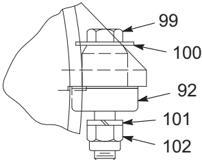
MOTOR MOUNT
