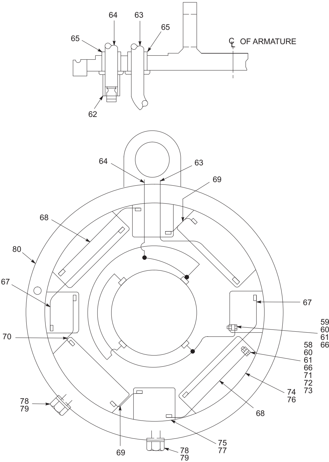
(Representative Illustration) FIG.4
