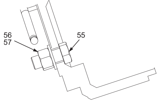
SECTION B-B (Representative Illustration) FIG. 3
