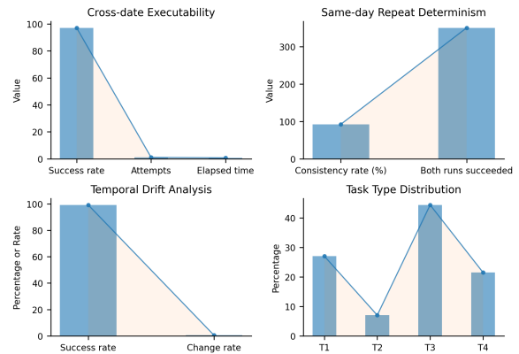
Figure 9: Code analysis experiments. We evaluate executability across dates, determinism across repeated runs, and temporal drift of time-sensitive tasks. High executability with non-trivial drift confirms that REALFIN captures realistic, time-varying financial environments.
