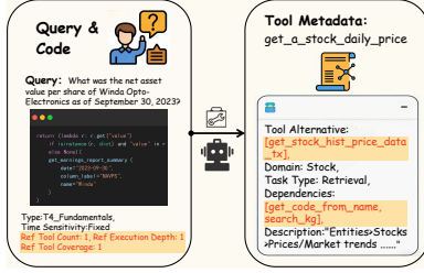
Figure 2: Data and tool structure in REALFIN. The left side illustrates the task-side representation including query text and executable code, while the right side shows the structured tool metadata such as domain, task type, dependencies, and alternatives.
