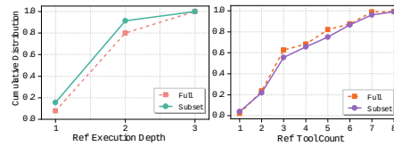
Figure 3: Structural similarity between the full benchmark and the 128-core subset.
