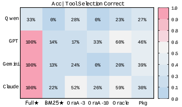
Figure 8: Conditional accuracy after tool selection. Accuracy improves sharply once the correct tools are selected, identifying tool choice as the primary bottleneck.
