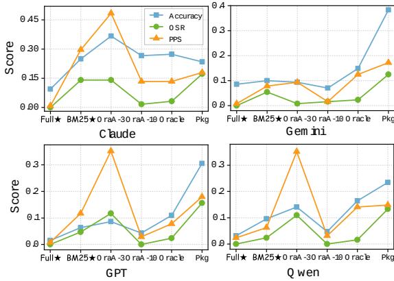
Figure 4: Effect of increasing flat-tool ambiguity. ACC, OSR, and PPS decline as the visible tool space moves from Oracle to alternatives, distractors, and Full exposure.
