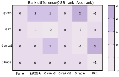
Figure 6: Rank-flip heatmap. ACC-based and OSR-based model rankings diverge across exposure regimes, revealing workflow failures hidden by answer-only scoring.
