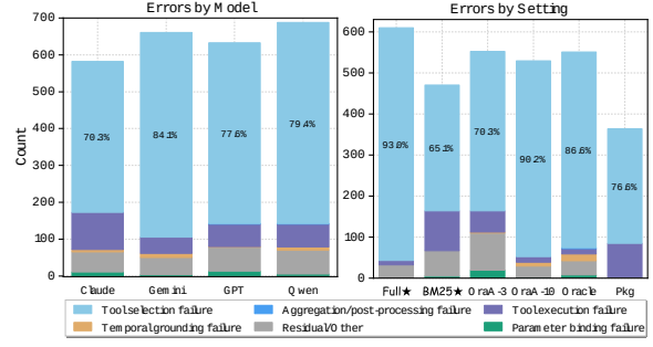
Figure 7: Error distribution. Most failures originate from incorrect tool selection and then cascade into downstream workflow errors.
