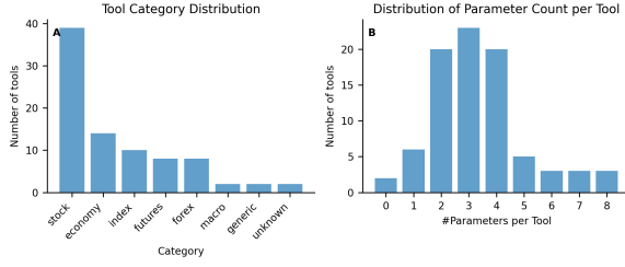
Figure 10: Tool ecosystem statistics. Left: distribution of tool categories. Right: distribution of parameter counts per tool. The benchmark exhibits heterogeneous and partially redundant tools, operationalizing the challenge of tool explosion.
