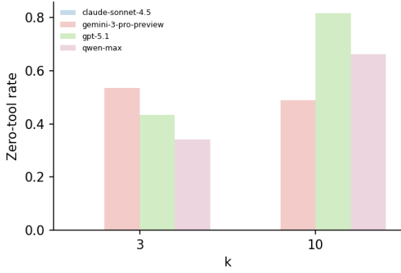
Figure 14: Zero-tool answer rate for k = 3 and k = 10 . Higher values indicate a stronger tendency to avoid tool usage entirely.
