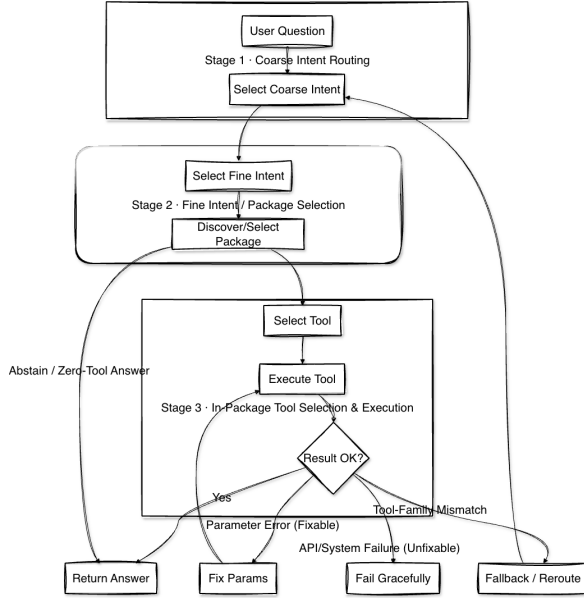
Figure 15: Hierarchical intent routing and packaged tool selection. The execution trace demonstrates that even when tools are grouped into packages, the agent must still disambiguate between multiple similar tools and coordinate multi-step workflows, indicating that tool explosion persists in packaged settings.
