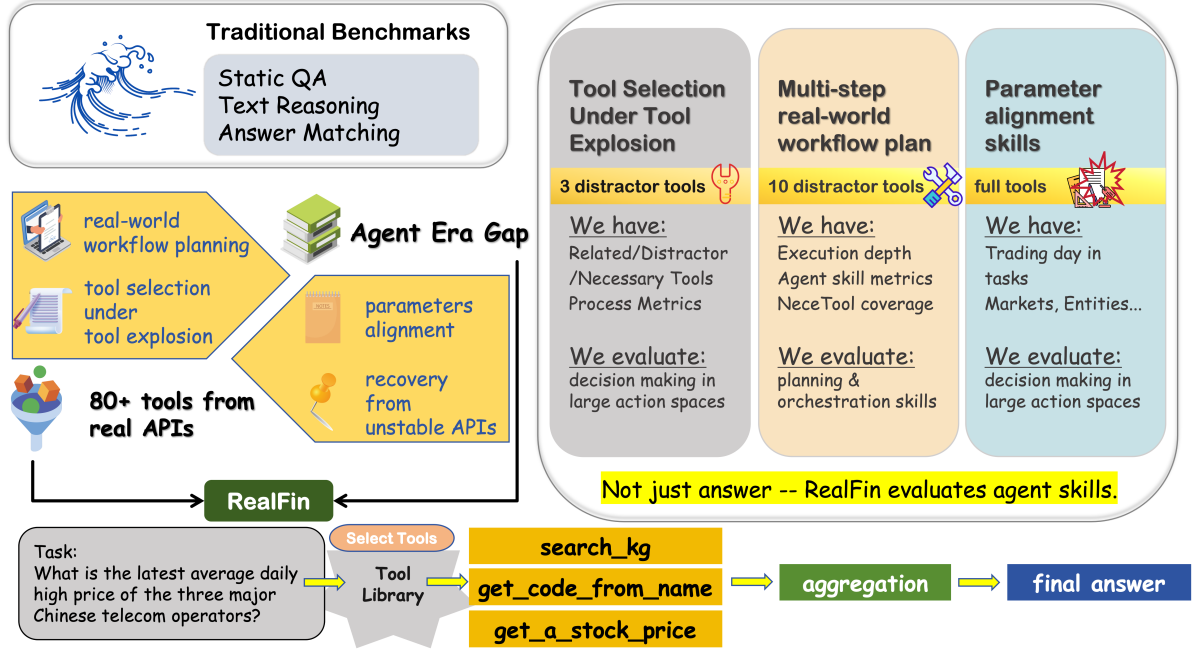
Figure 1: Overall concept of REALFIN: workflow-grounded financial tasks, executable golden code, and a realistic multi-tool environment where flat tool exposure leads to tool explosion.
