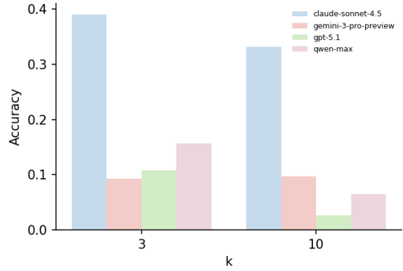
Figure 12: Accuracy comparison between k = 3 and k = 10 on the 394-item paired subset. Each bar shows mean accuracy across samples for each model.
