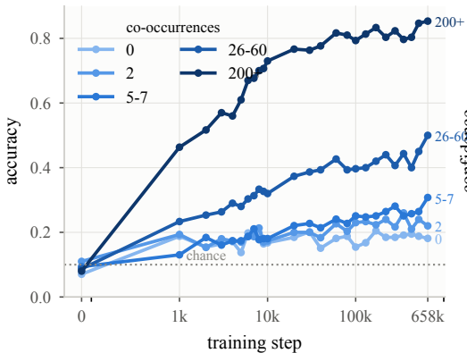
accuracy separates across the whole range
