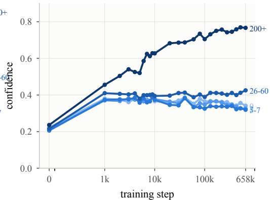
confidence separates only for the most frequent facts
