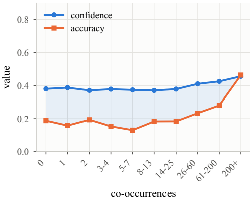
step 1,000
