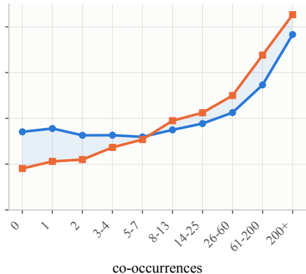
step 658,032 (final)
