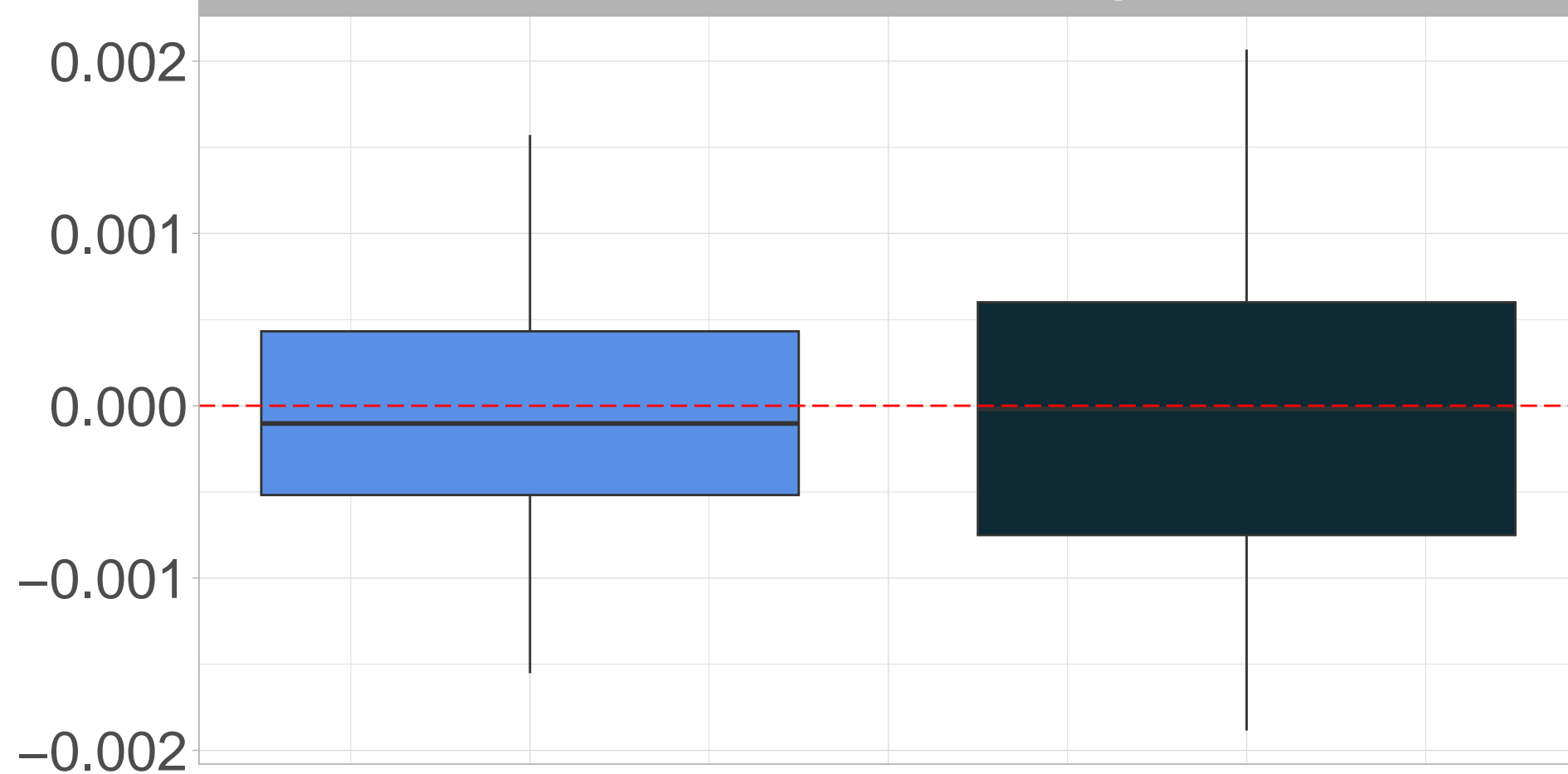
Linear Reg. Coef ( \theta ) Caliper Matching
