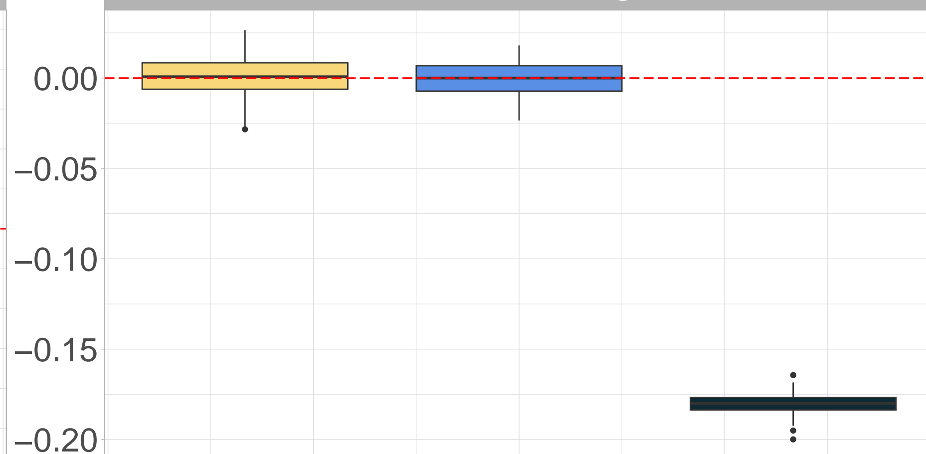
Cond. Survival NN Matching
