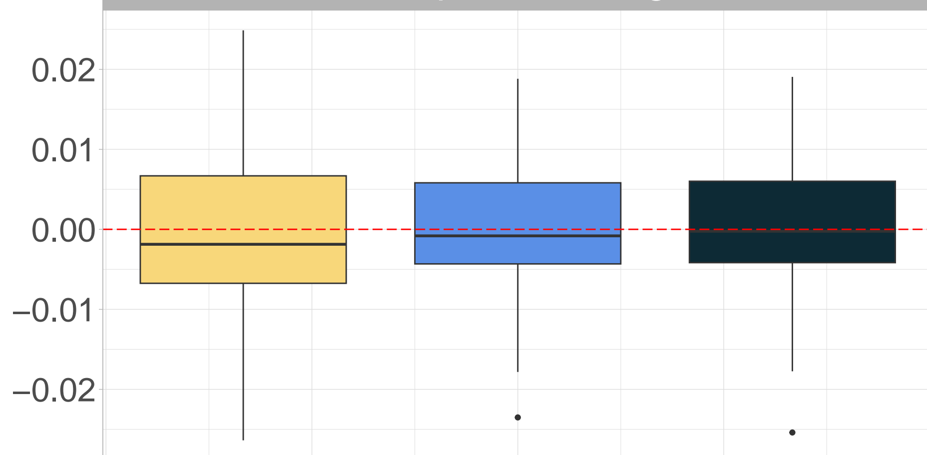
Cond. Survival Caliper Matching
