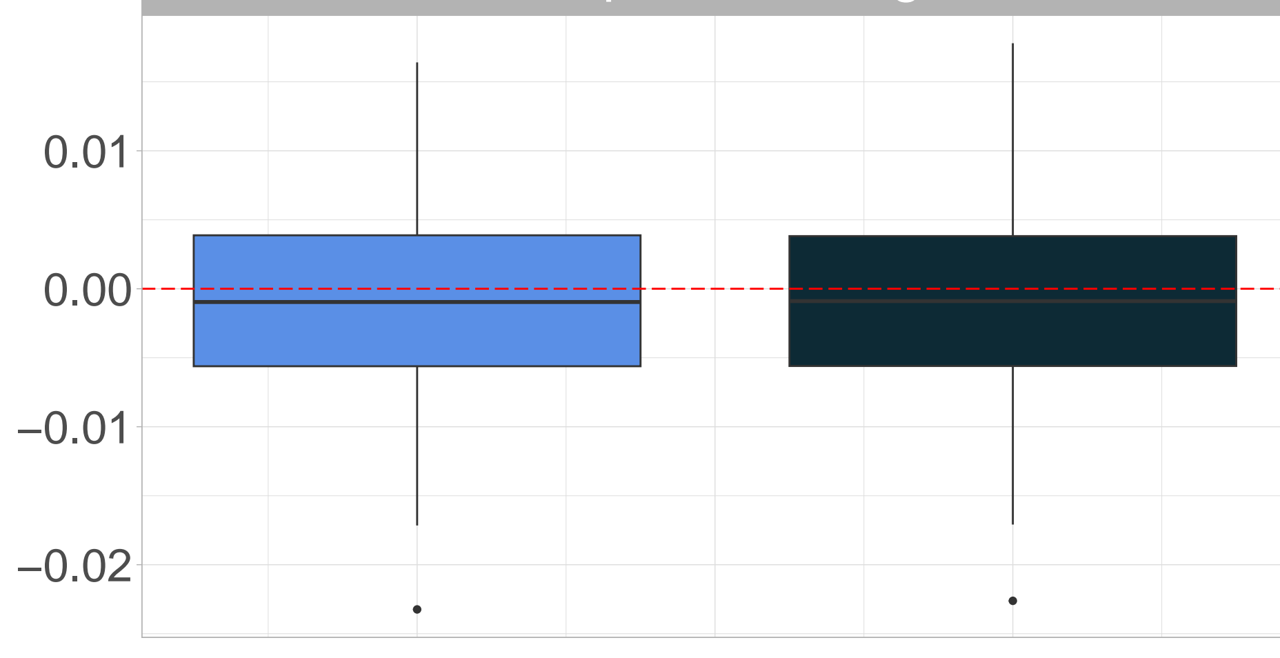
Linear Reg. Coef ( \theta ) Caliper Matching
