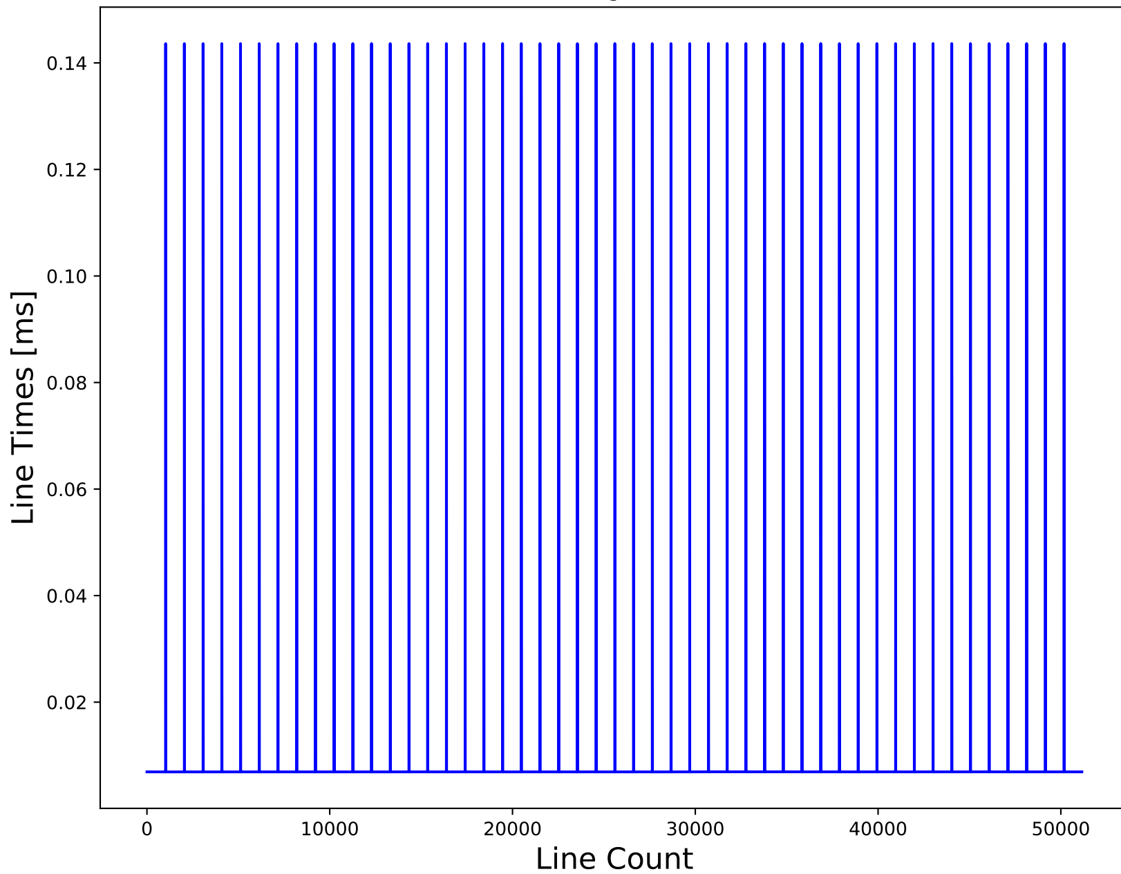
Variation of Line Times during Backwards Scan (Coumarin)
