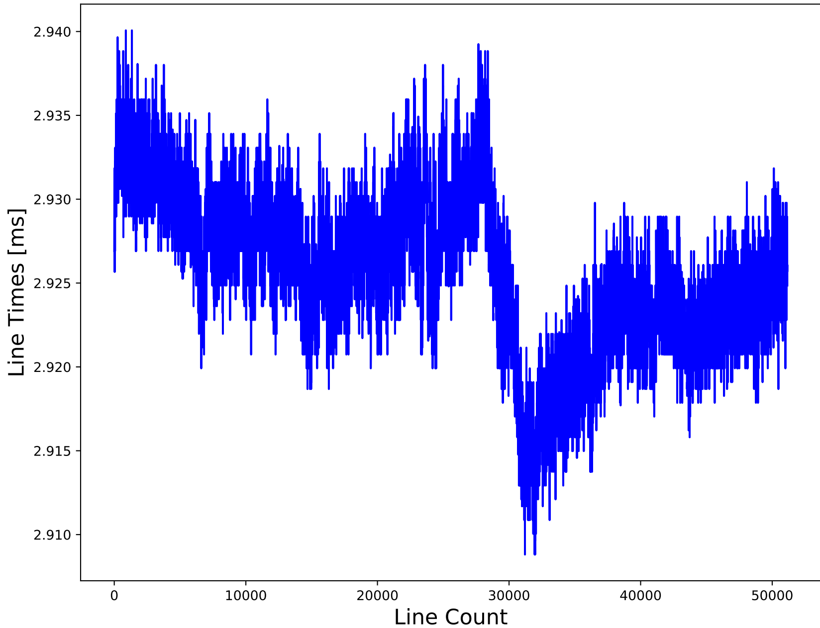
Variation of Line Times during Forward Scan (Coumarin)
