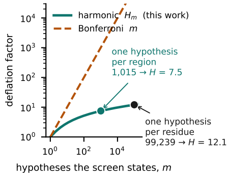
a Arbitrary dependence costs a logarithm, not a factor of m
