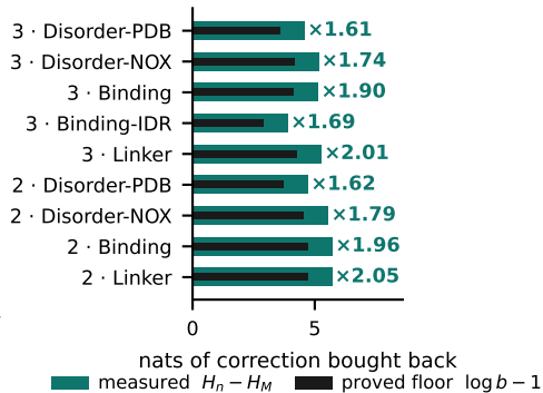
b Testing regions, not residues (label = threshold gained)
