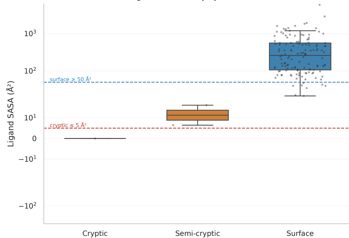
Ligand accessibility by burial class
