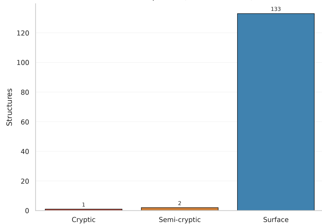
Dataset composition (n=136 structures)
