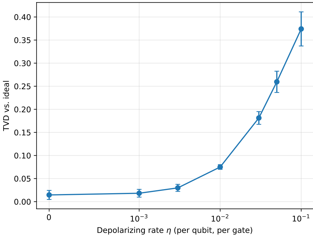
Noise robustness (N=64, M=2000)
