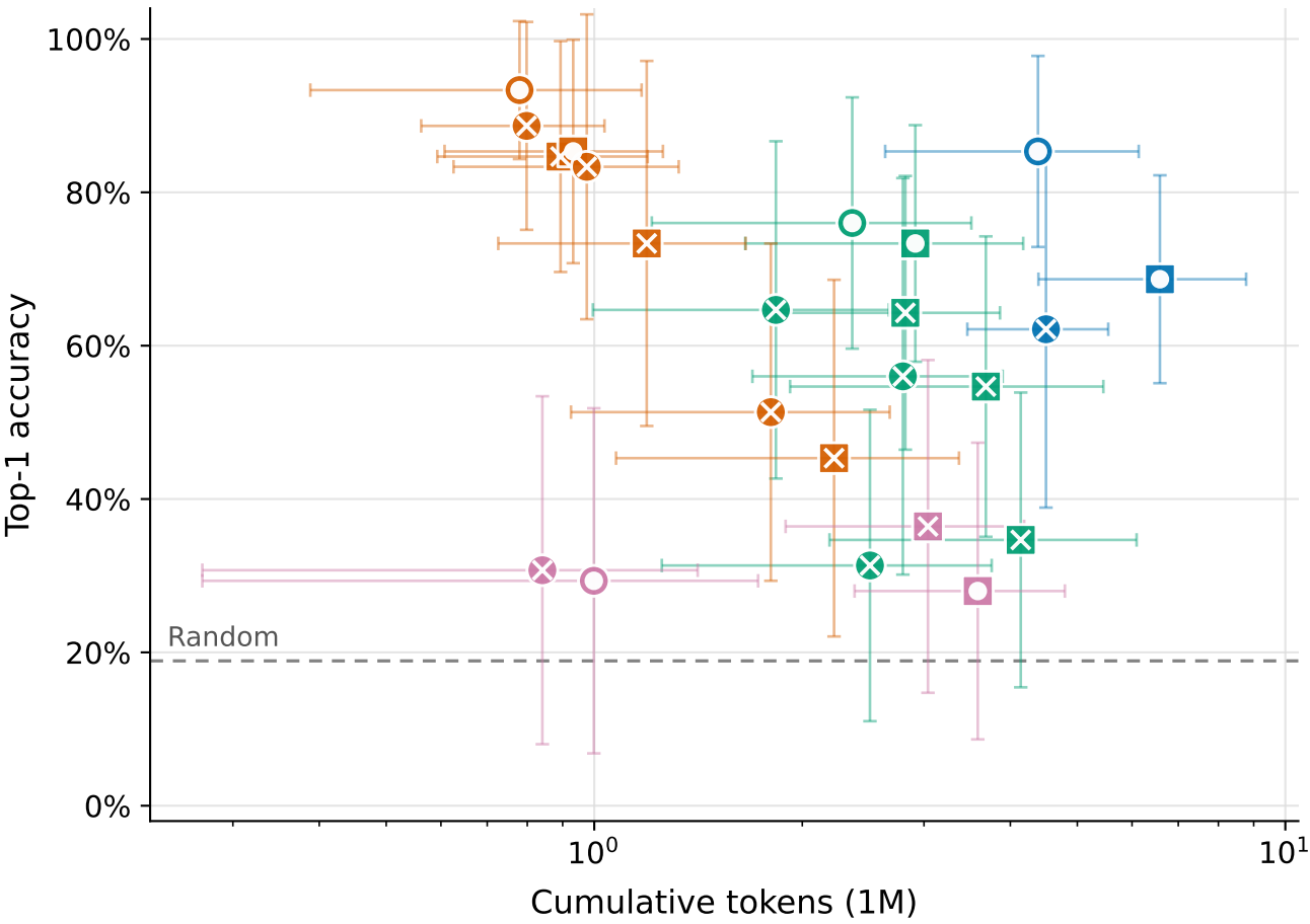
Accuracy vs. token usage
