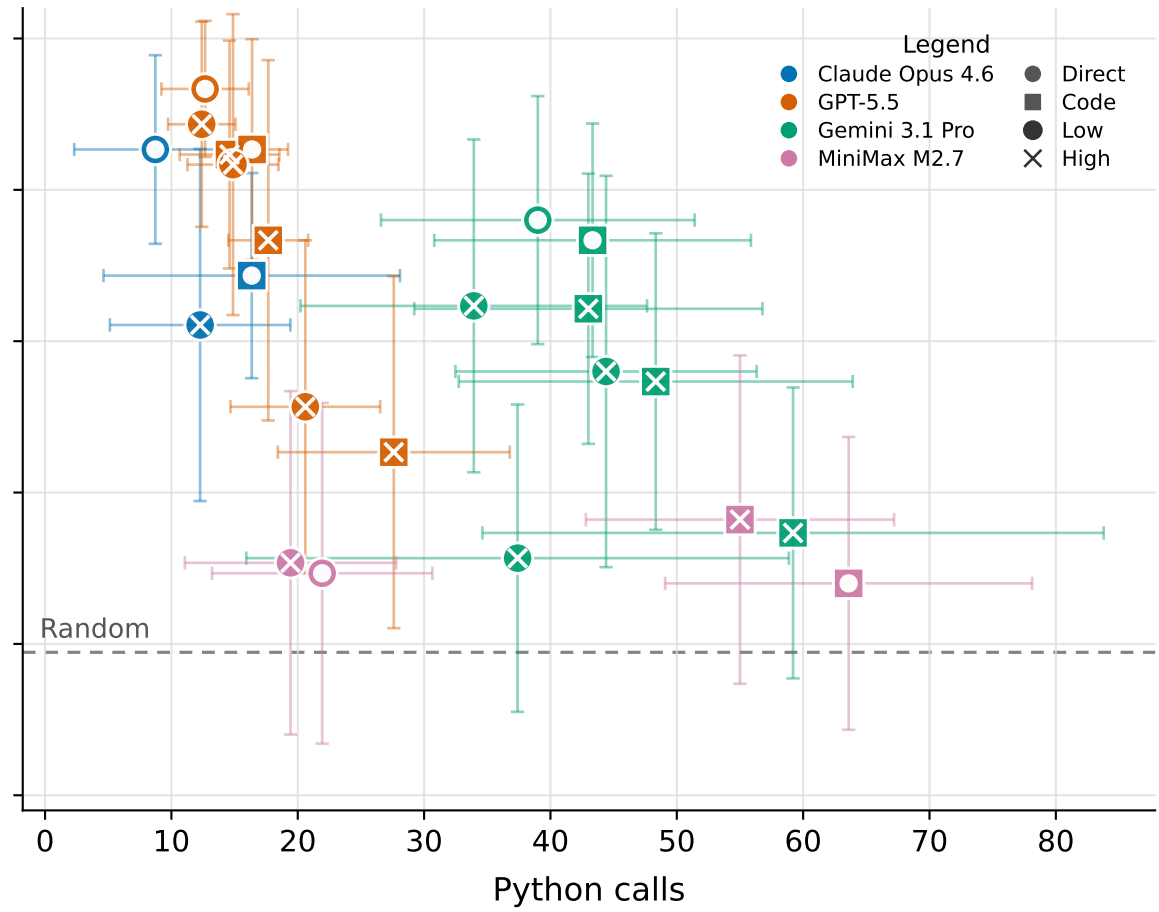
Accuracy vs. Python calls
