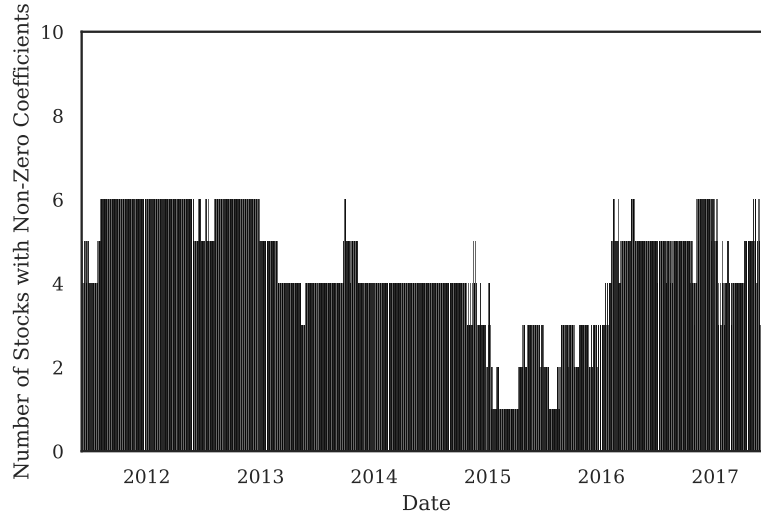
Figure 1: Number of Stocks with Non-Zero Coefficients Over Time
