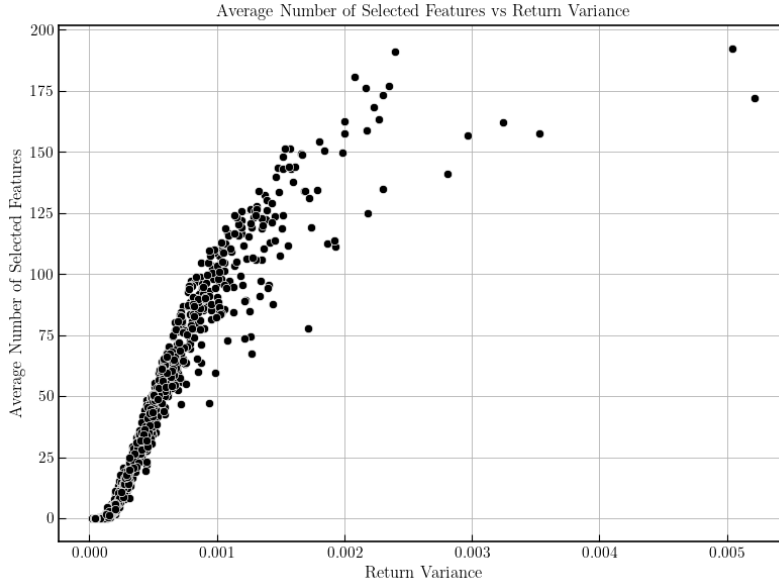
Figure 1: Average Number of Non-Zero Coefficients vs. Return Variance
