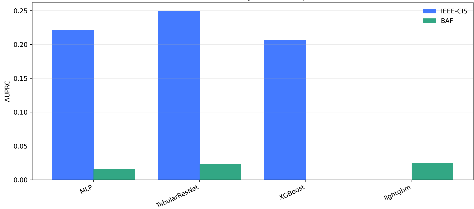
Locked-test AUPRC by dataset and predictor
