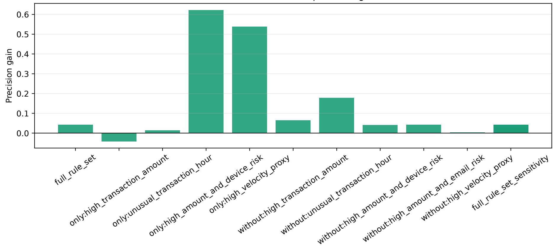
IEEE-CIS rule ablation precision gain
