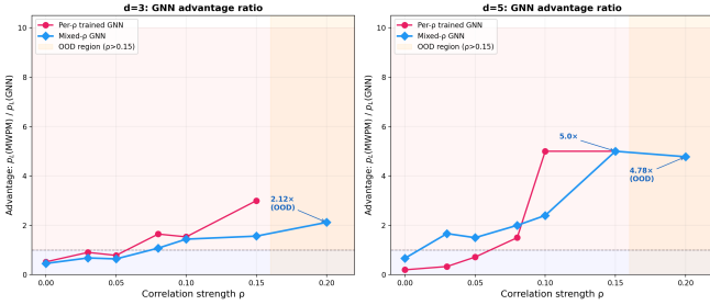
FIG. 4. GNN advantage ratio p_L(\text{MWPM})/p_L(\text{GNN}) vs. inter-mode correlation \rho . Left: d=3 . Right: d=5 . Values above the dashed line indicate GNN outperforms MWPM. The shaded region ( \rho > 0.15 ) is out of the GNN training distribution. The GNN advantage increases from d=3 to d=5 , in contrast to the typical scaling behavior of ML decoders.
