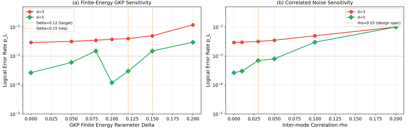
FIG. 3. Robustness analysis at Phase 1 parameters ( \sigma_{\text{eff}} = 8.5 dB). (a) Impact of finite-energy GKP parameter \Delta : for \Delta \leq 0.12 (design target), the degradation is modest ( 1.6\text{--}1.8\times ). (b) Impact of inter-mode correlation \rho : at design spec \rho \leq 0.03 , impact is negligible; MWPM performance degrades noticeably at \rho \geq 0.08 .
