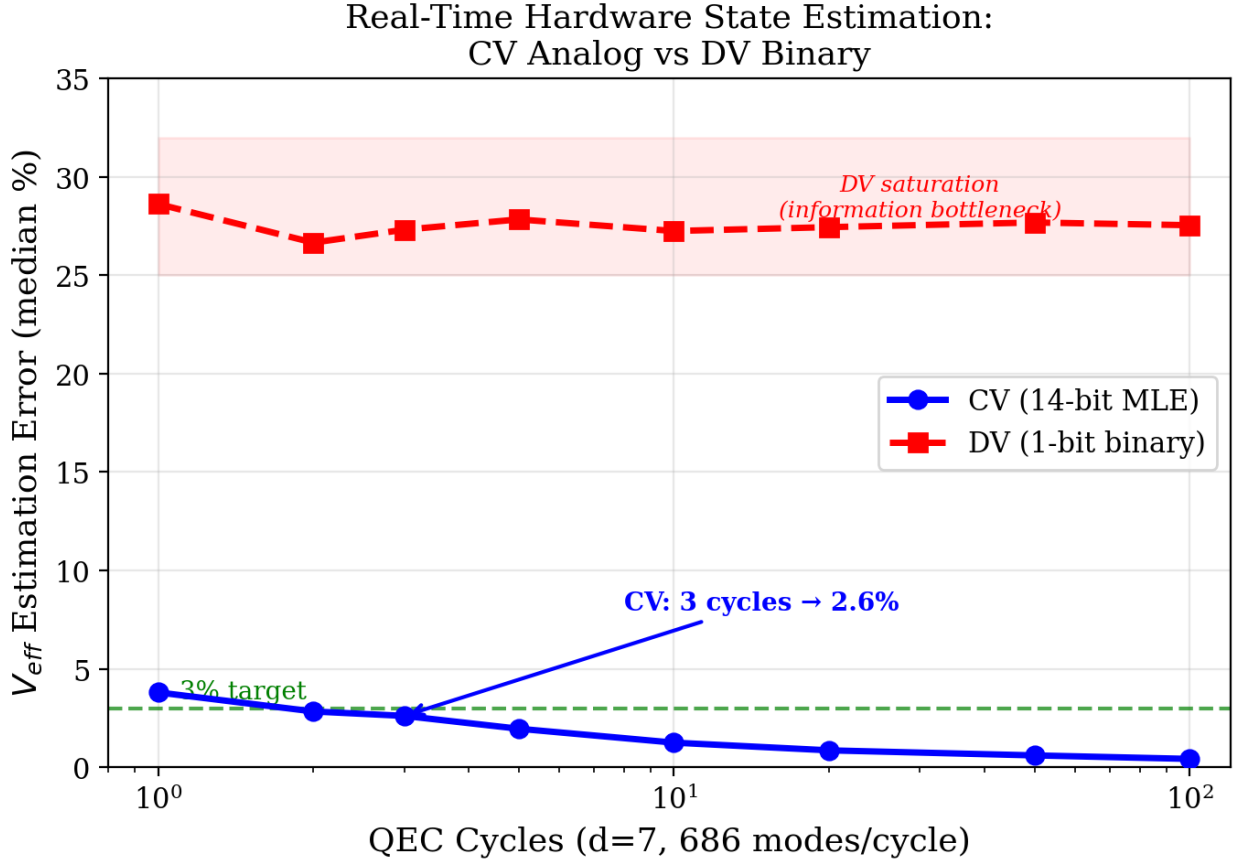
Figure 3. V_{eff} estimation error vs QEC cycle count. CV (blue) achieves 3% accuracy in 3 cycles. DV (red) saturates at 28% even after 100 cycles due to information bottleneck.
