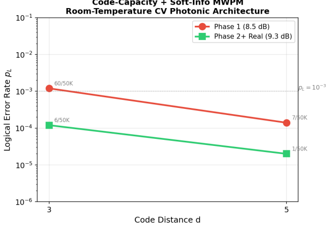
FIG. 1. Logical error rate p_L vs. code distance d for two operating points (code-capacity + soft-info MWPM). Error counts annotated. Exponential suppression confirms operation below threshold.
