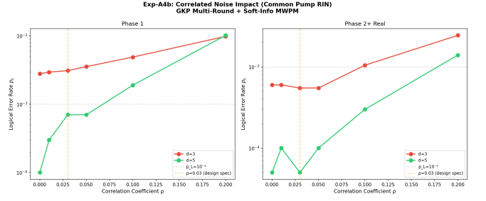
FIG. 4. Impact of inter-mode correlation \rho on logical error rates.
