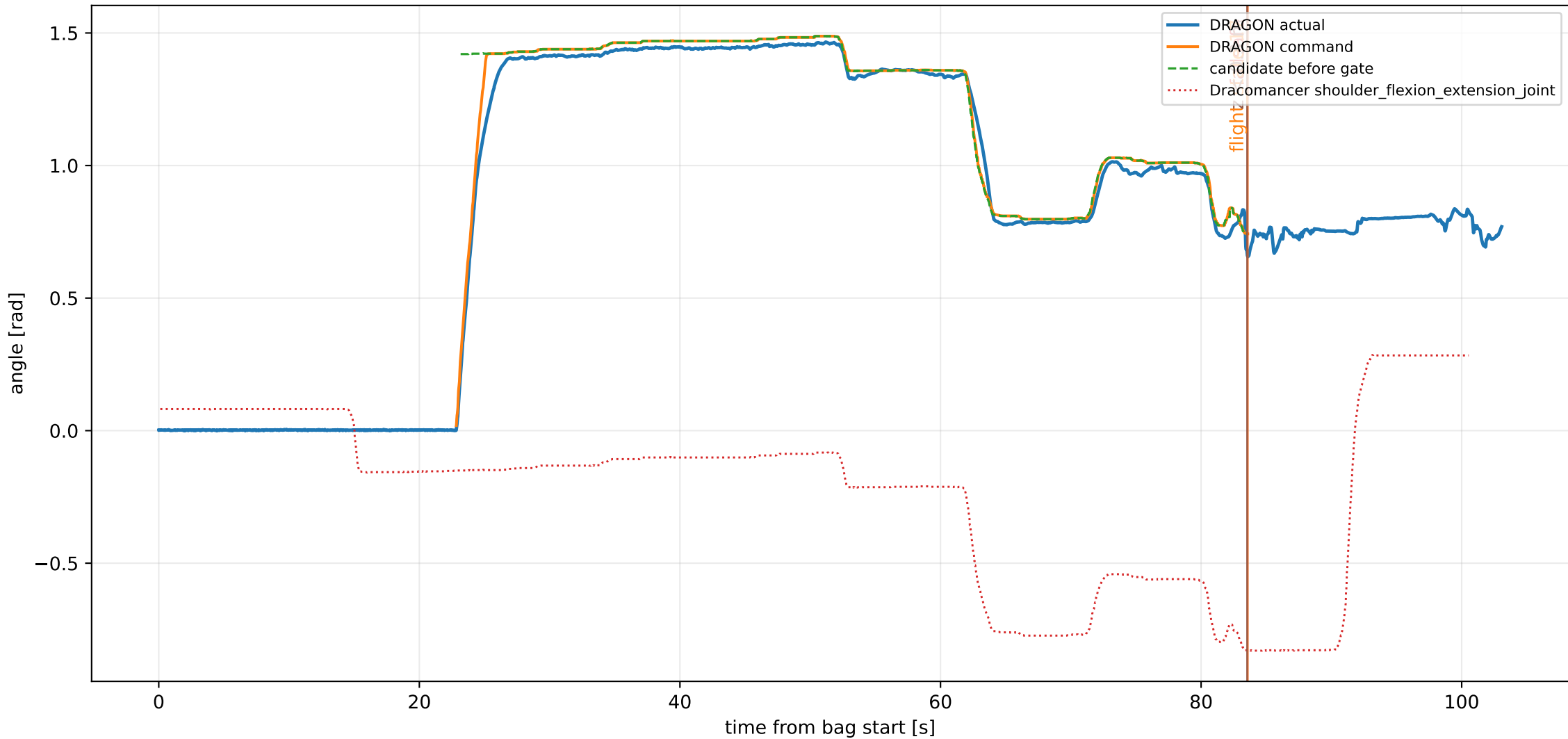
joint3_pitch mapping trace
