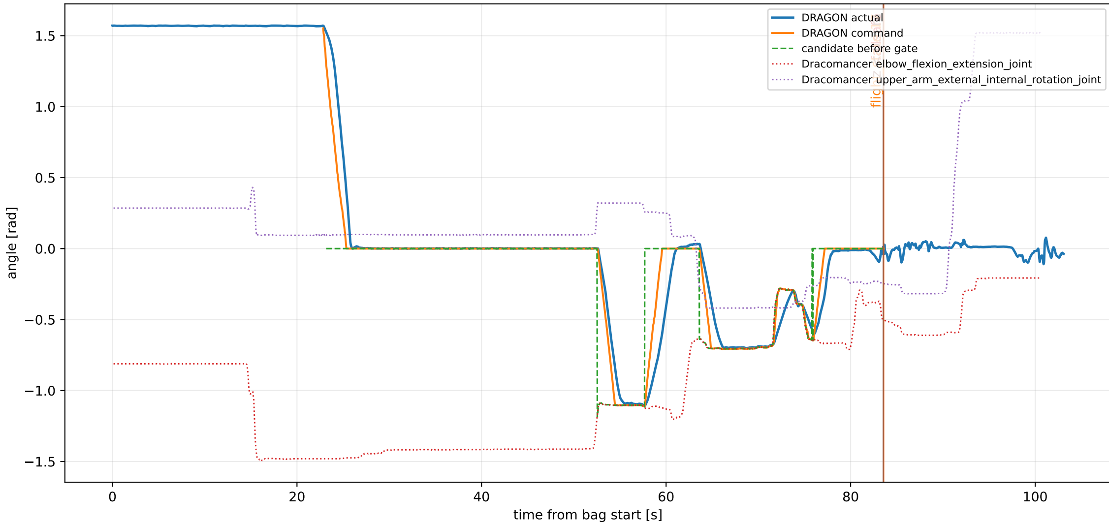
joint2_yaw mapping trace
