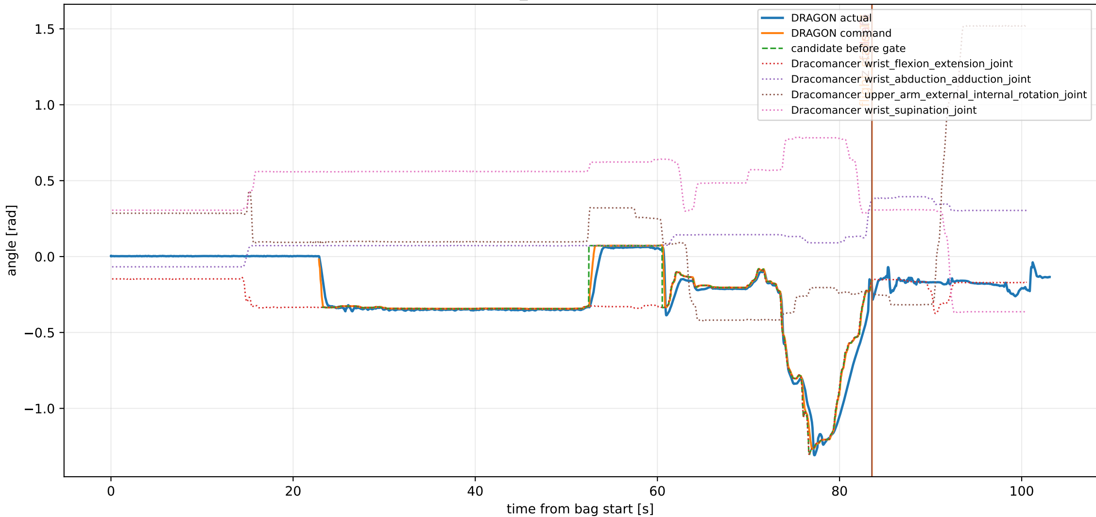
joint1_pitch mapping trace
