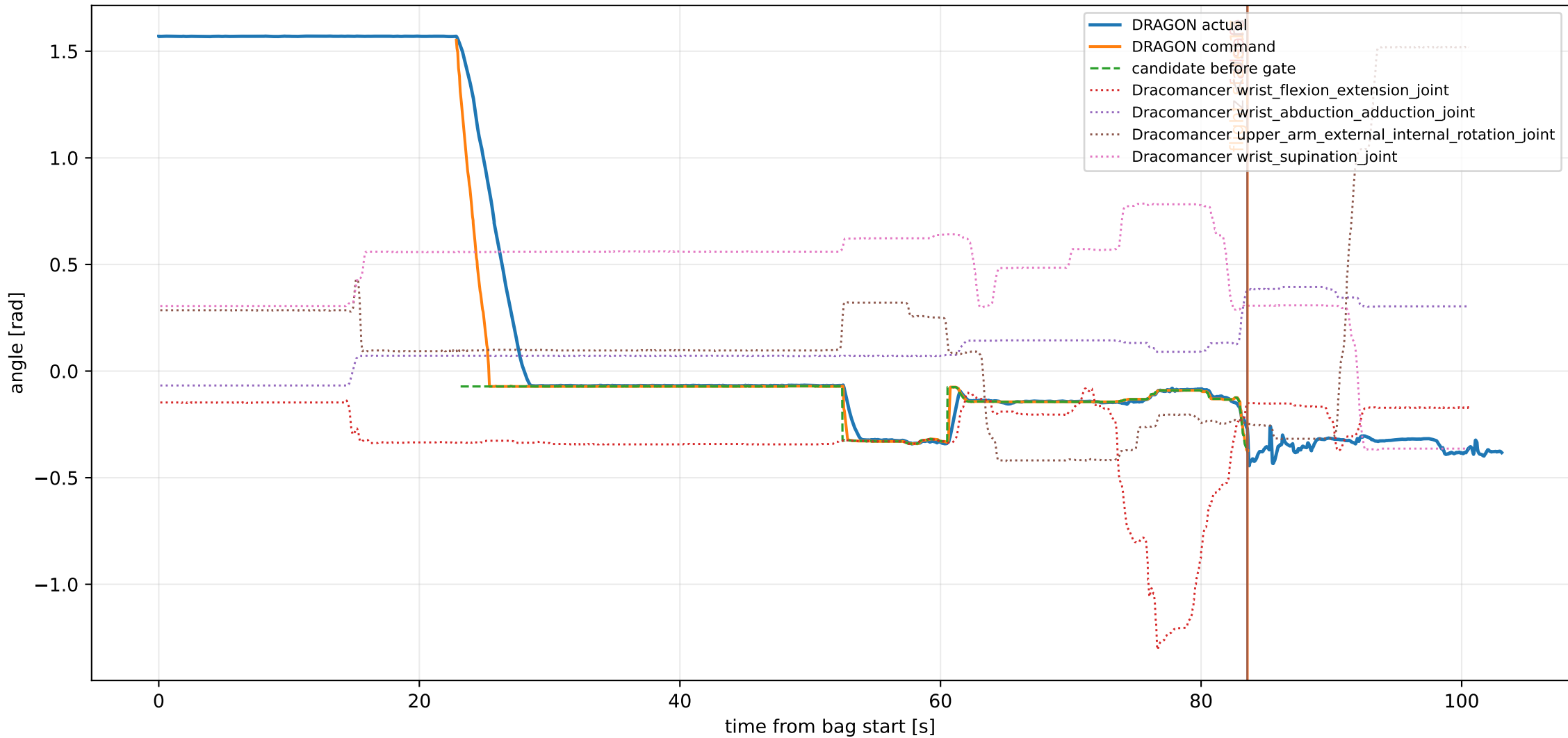
joint1_yaw mapping trace
