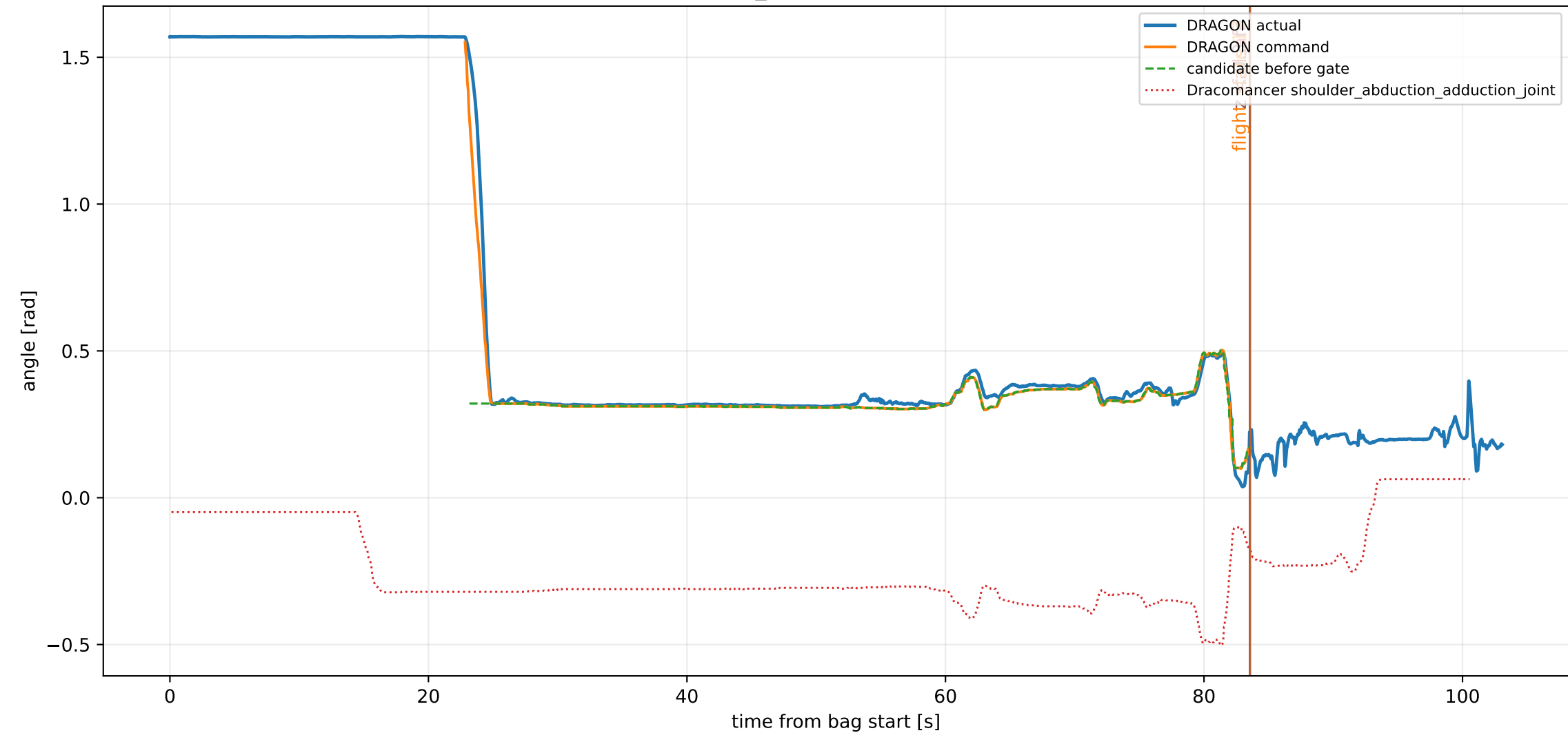
joint3_yaw mapping trace
